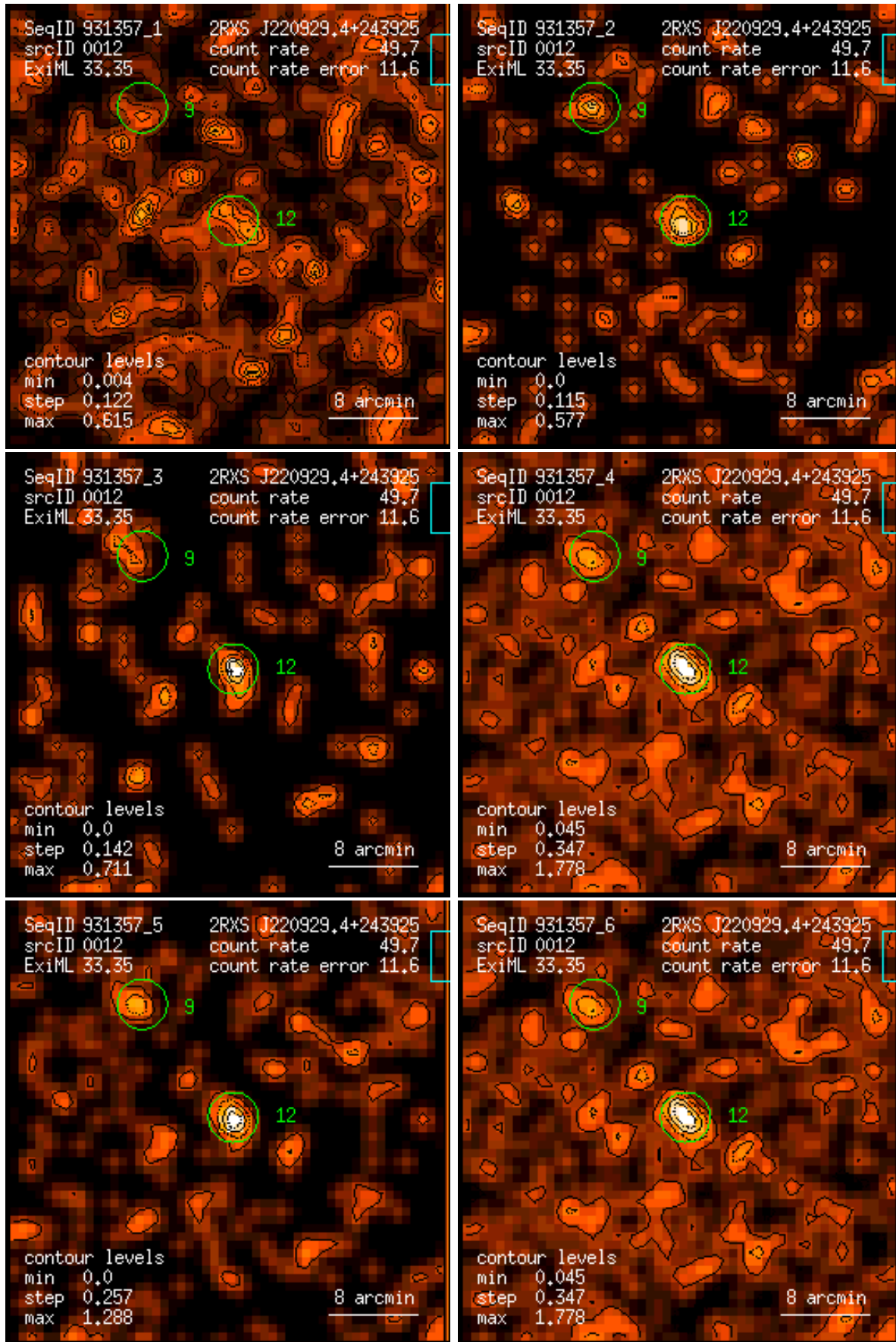
Figure 12: RASS 931357: detection 0012: band rate images, Gaussian filter: (1) PSPC channels 11 – 41, (2) 52 – 90, (3) 91 – 201, (4) 11 – 235, (5) 52 – 201, (6) 11 – 201. Broad band rates in counts/ks. Band rate contour levels in counts/ks/arcmin 2 .
