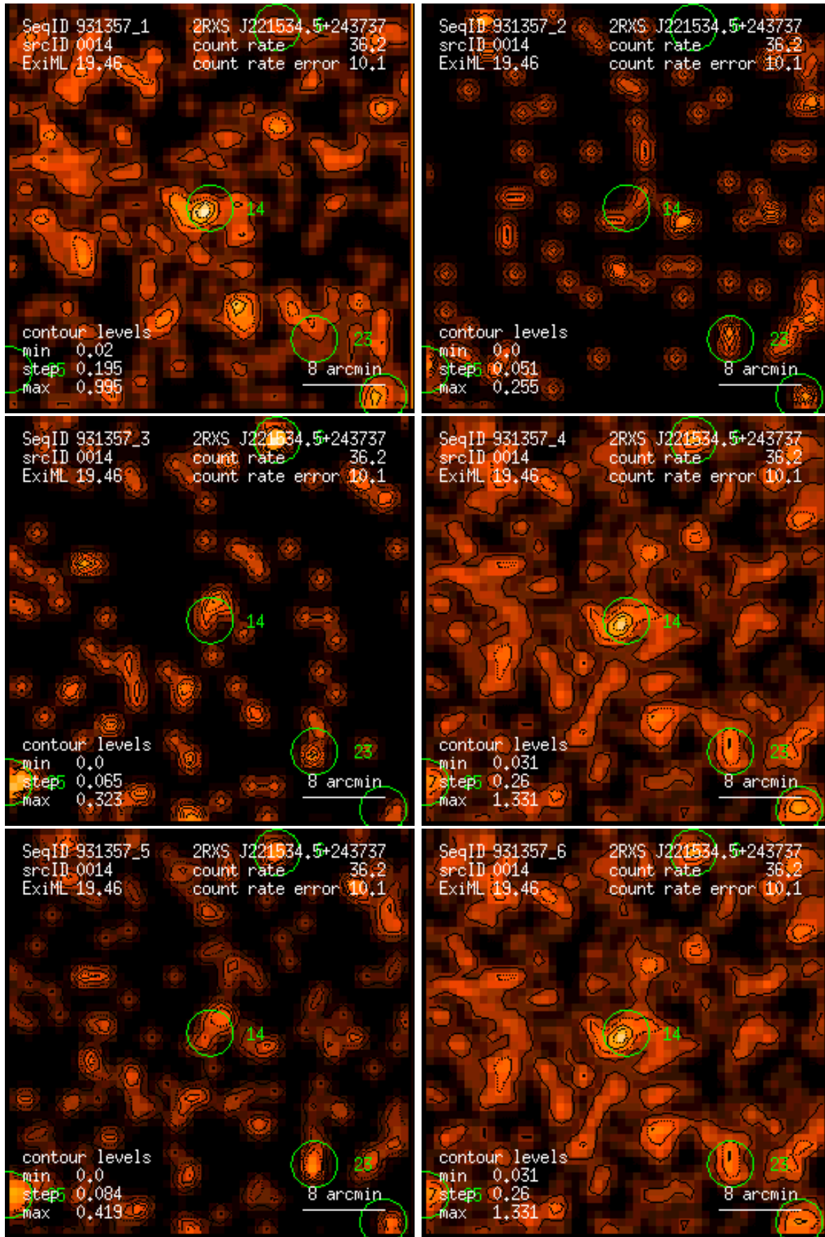
Figure 14: RASS 931357: detection 0014: band rate images, Gaussian filter: (1) PSPC channels 11 – 41, (2) 52 – 90, (3) 91 – 201, (4) 11 – 235, (5) 52 – 201, (6) 11 – 201. Broad band rates in counts/ks. Band rate contour levels in counts/ks/arcmin 2 .
