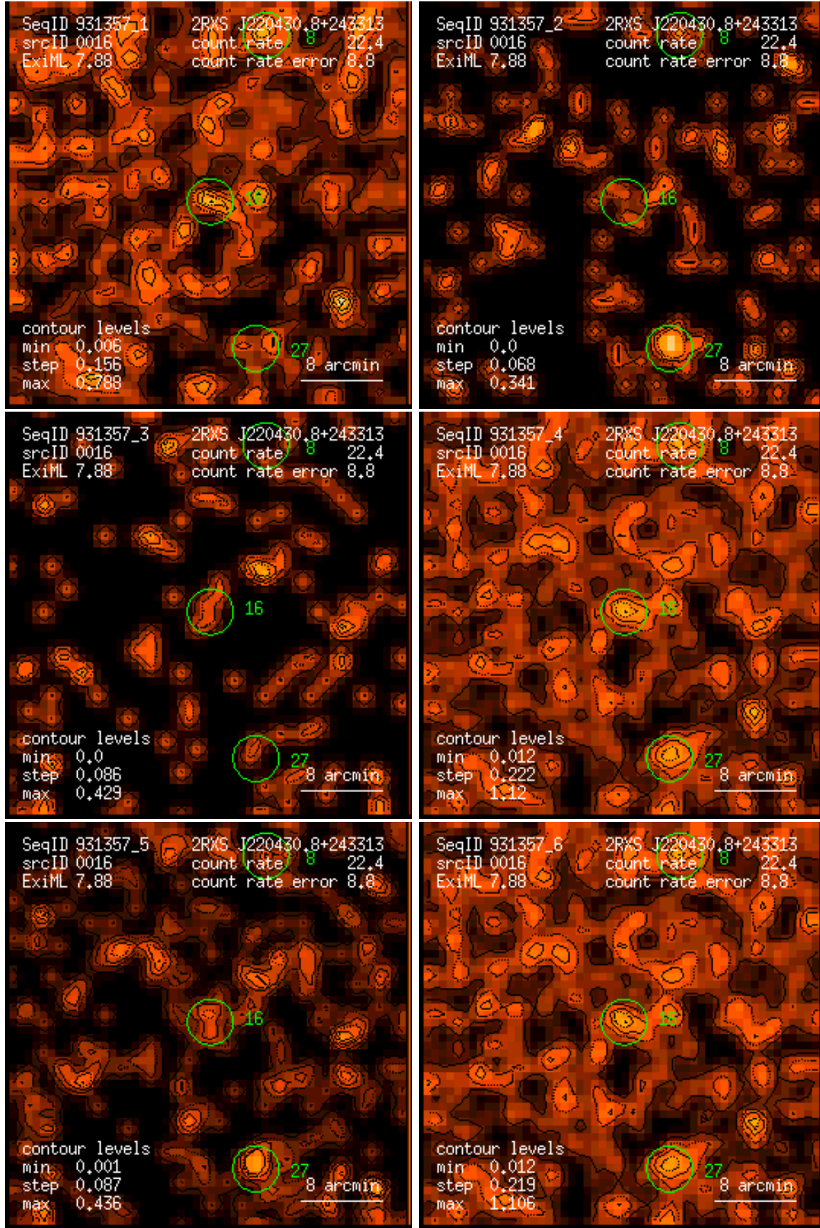
Figure 16: RASS 931357: detection 0016: band rate images, Gaussian filter: (1) PSPC channels 11 – 41, (2) 52 – 90, (3) 91 – 201, (4) 11 – 235, (5) 52 – 201, (6) 11 – 201. Broad band rates in counts/ks. Band rate contour levels in counts/ks/arcmin 2 .
