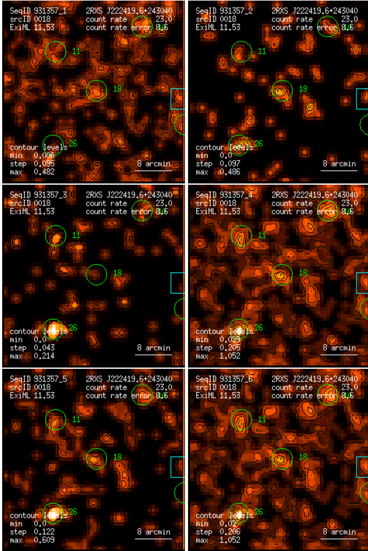
Figure 18: RASS 931357: detection 0018: band rate images, Gaussian filter: (1) PSPC channels 11 – 41, (2) 52 – 90, (3) 91 – 201, (4) 11 – 235, (5) 52 – 201, (6) 11 – 201. Broad band rates in counts/ks. Band rate contour levels in counts/ks/arcmin 2 .
