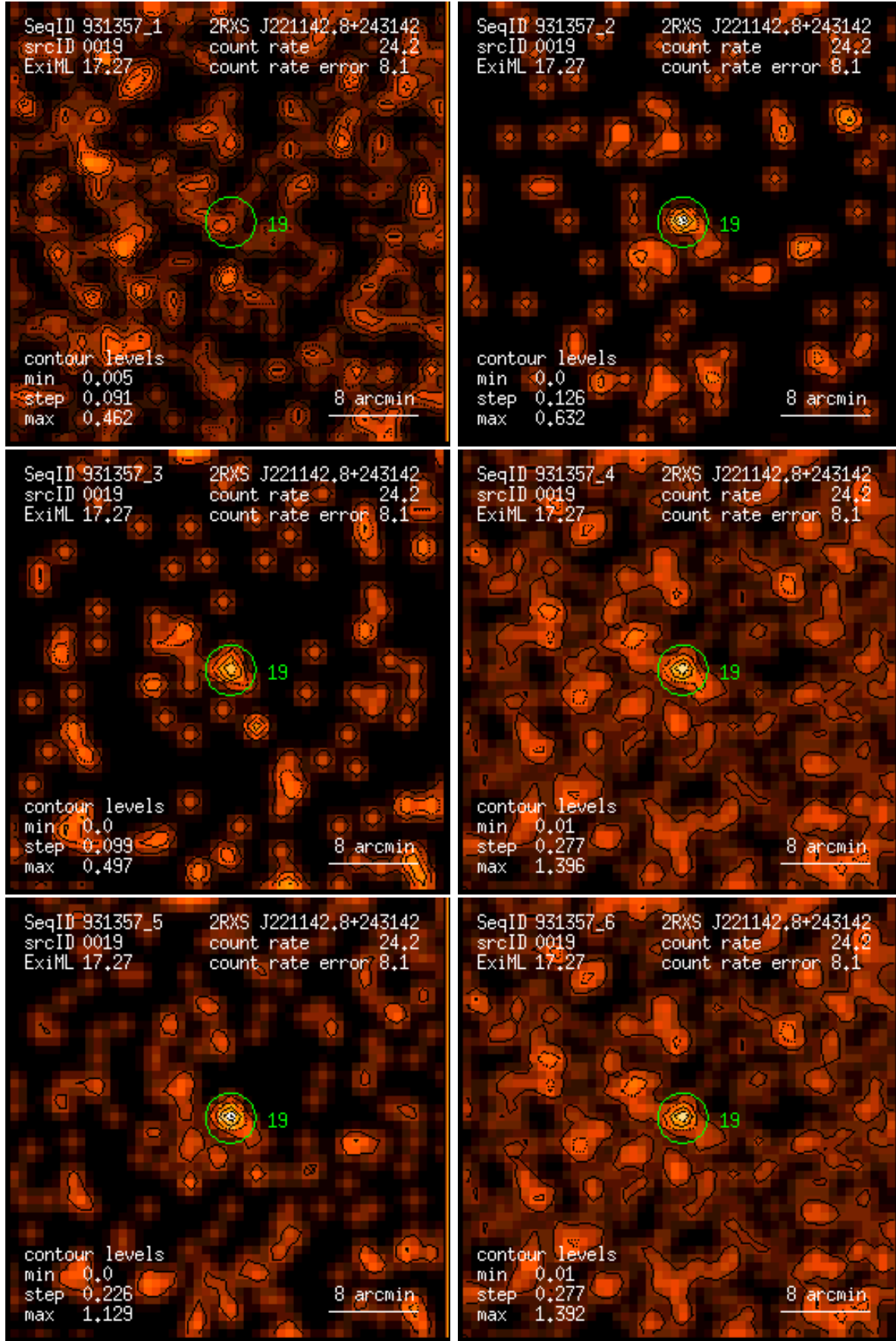
Figure 19: RASS 931357: detection 0019: band rate images, Gaussian filter: (1) PSPC channels 11 – 41, (2) 52 – 90, (3) 91 – 201, (4) 11 – 235, (5) 52 – 201, (6) 11 – 201. Broad band rates in counts/ks. Band rate contour levels in counts/ks/arcmin 2 .
