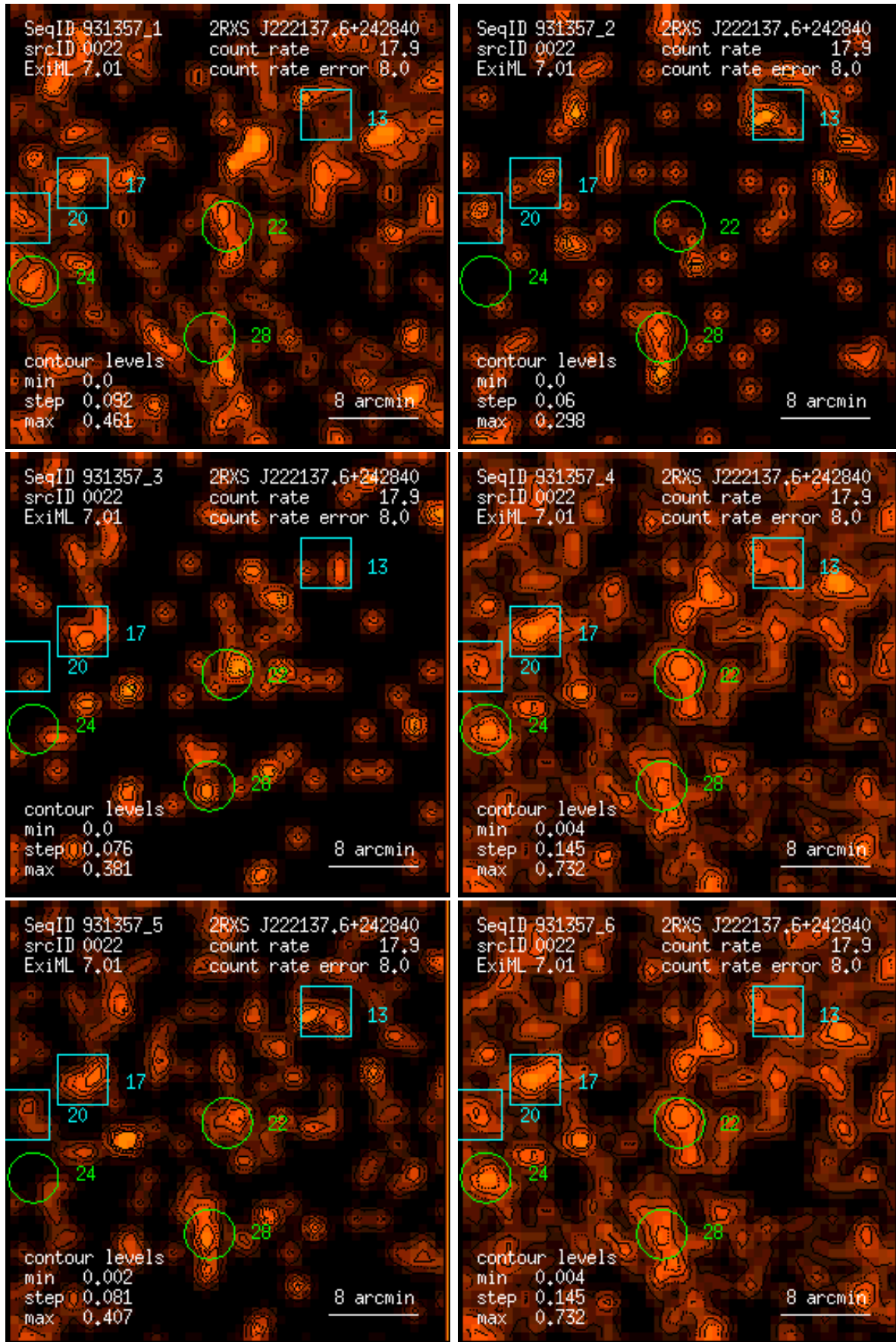
Figure 22: RASS 931357: detection 0022: band rate images, Gaussian filter: (1) PSPC channels 11 – 41, (2) 52 – 90, (3) 91 – 201, (4) 11 – 235, (5) 52 – 201, (6) 11 – 201. Broad band rates in counts/ks. Band rate contour levels in counts/ks/arcmin 2 .
