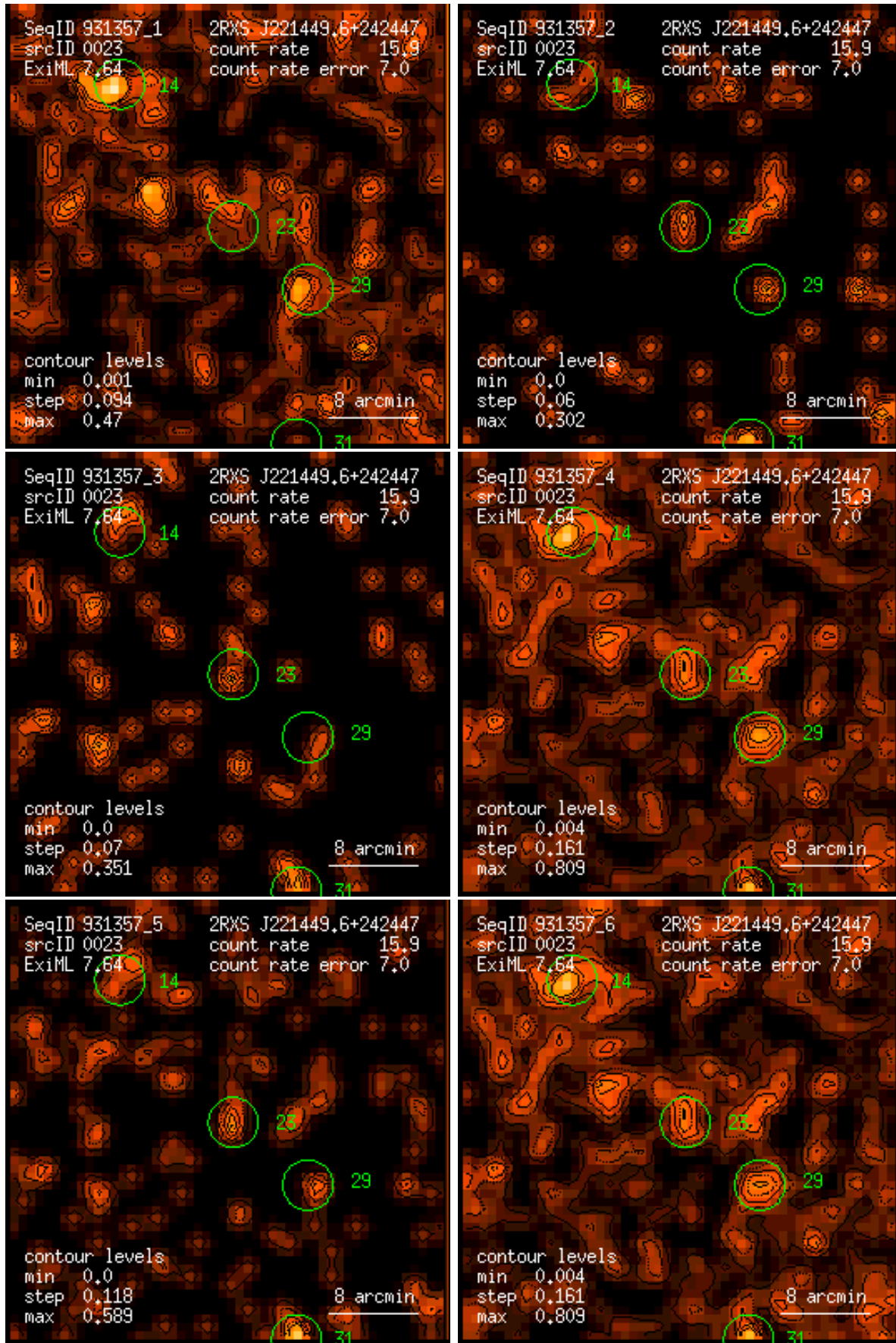
Figure 23: RASS 931357: detection 0023: band rate images, Gaussian filter: (1) PSPC channels 11 – 41, (2) 52 – 90, (3) 91 – 201, (4) 11 – 235, (5) 52 – 201, (6) 11 – 201. Broad band rates in counts/ks. Band rate contour levels in counts/ks/arcmin 2 .
