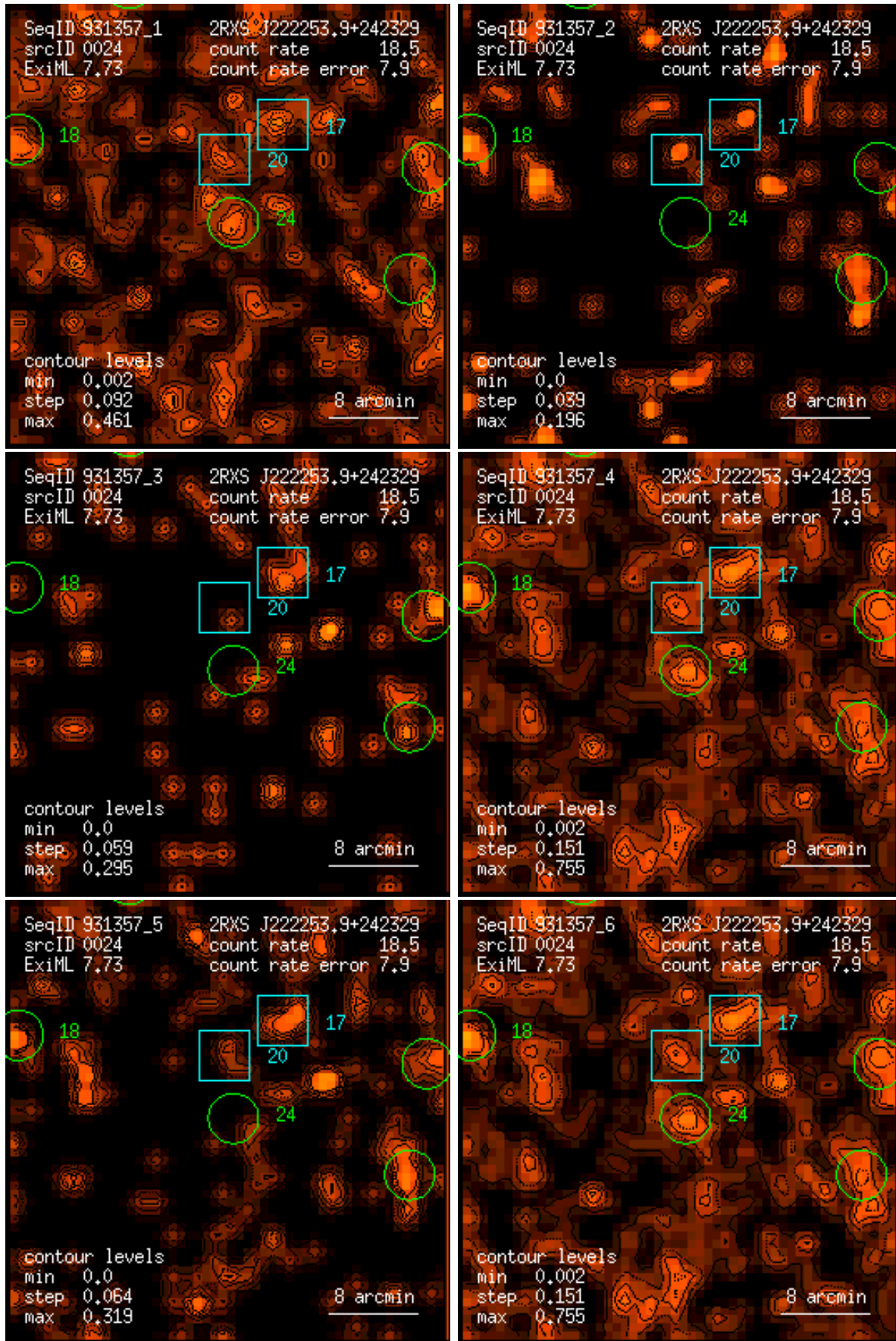
Figure 24: RASS 931357: detection 0024: band rate images, Gaussian filter: (1) PSPC channels 11 – 41, (2) 52 – 90, (3) 91 – 201, (4) 11 – 235, (5) 52 – 201, (6) 11 – 201. Broad band rates in counts/ks. Band rate contour levels in counts/ks/arcmin 2 .
