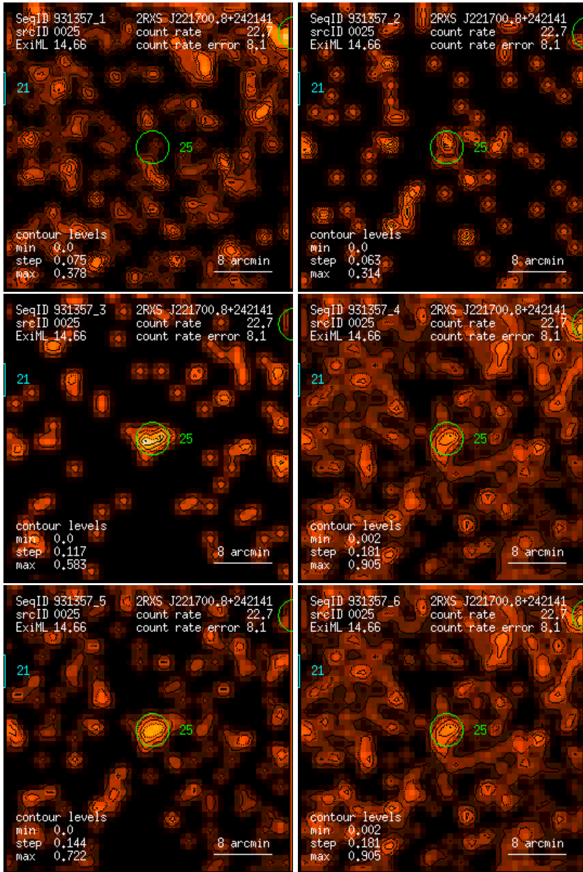
Figure 25: RASS 931357: detection 0025: band rate images, Gaussian filter: (1) PSPC channels 11 – 41, (2) 52 – 90, (3) 91 – 201, (4) 11 – 235, (5) 52 – 201, (6) 11 – 201. Broad band rates in counts/ks. Band rate contour levels in counts/ks/arcmin 2 .
