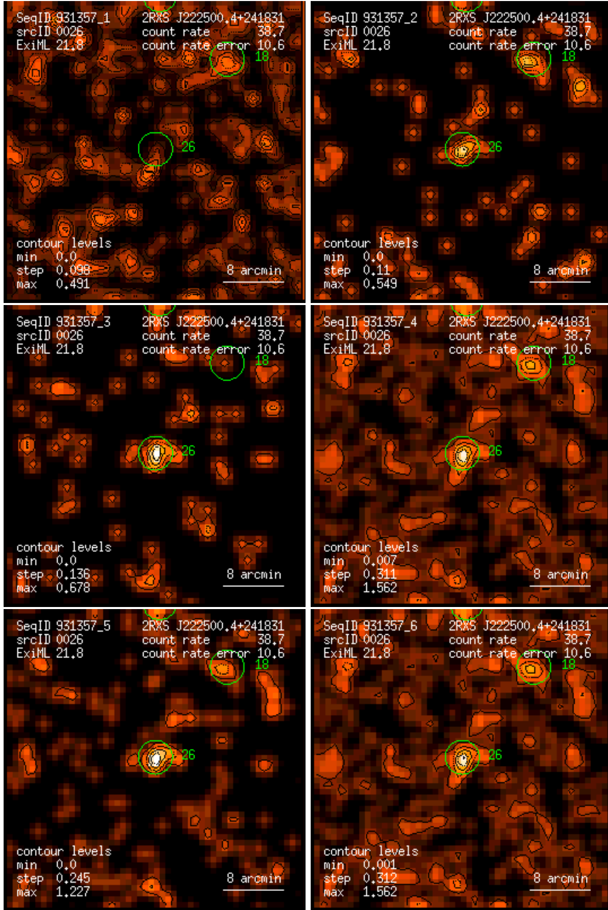
Figure 26: RASS 931357: detection 0026: band rate images, Gaussian filter: (1) PSPC channels 11 – 41, (2) 52 – 90, (3) 91 – 201, (4) 11 – 235, (5) 52 – 201, (6) 11 – 201. Broad band rates in counts/ks. Band rate contour levels in counts/ks/arcmin 2 .
