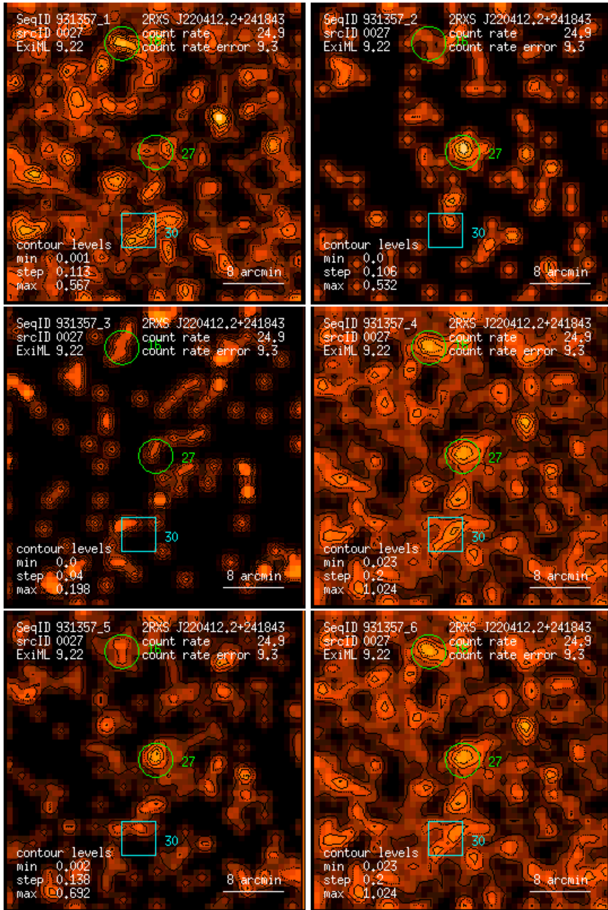
Figure 27: RASS 931357: detection 0027: band rate images, Gaussian filter: (1) PSPC channels 11 – 41, (2) 52 – 90, (3) 91 – 201, (4) 11 – 235, (5) 52 – 201, (6) 11 – 201. Broad band rates in counts/ks. Band rate contour levels in counts/ks/arcmin 2 .
