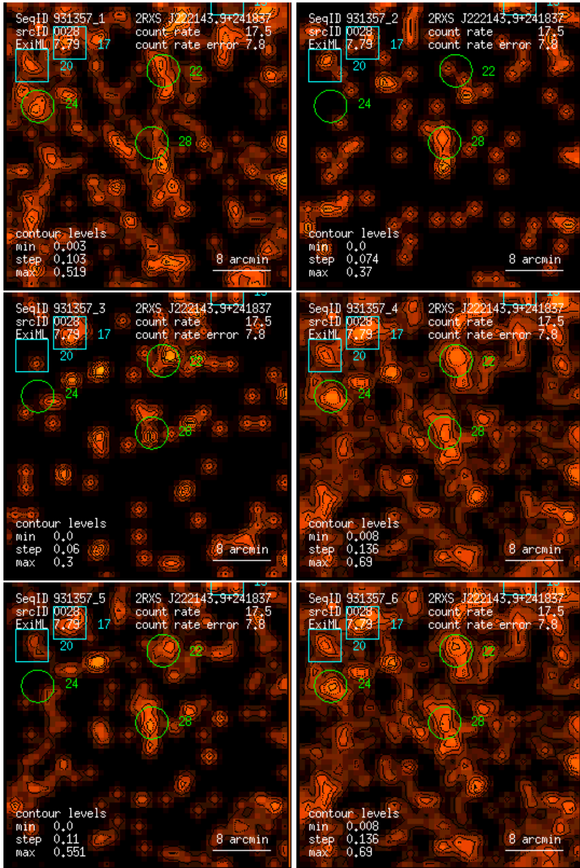
Figure 28: RASS 931357: detection 0028: band rate images, Gaussian filter: (1) PSPC channels 11 – 41, (2) 52 – 90, (3) 91 – 201, (4) 11 – 235, (5) 52 – 201, (6) 11 – 201. Broad band rates in counts/ks. Band rate contour levels in counts/ks/arcmin 2 .
