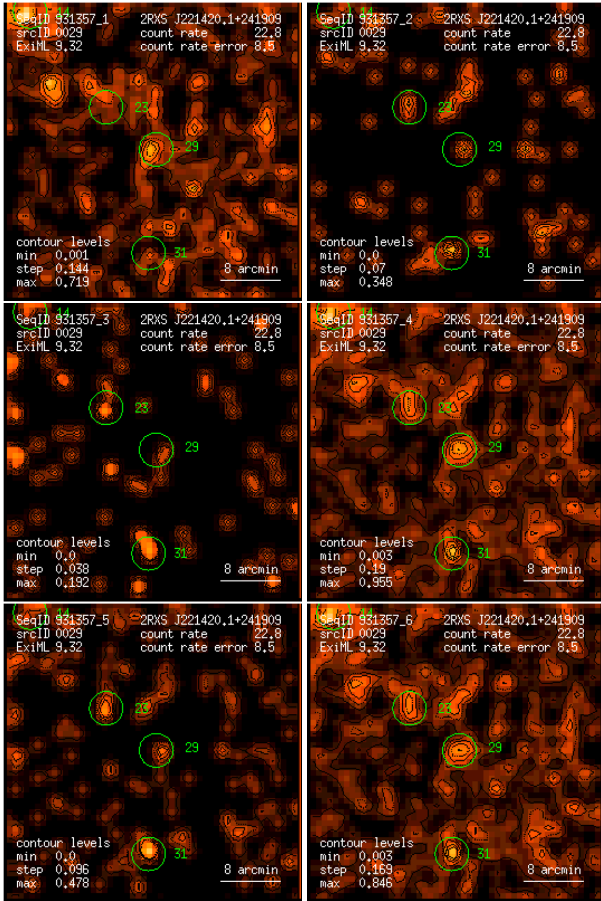
Figure 29: RASS 931357: detection 0029: band rate images, Gaussian filter: (1) PSPC channels 11 – 41, (2) 52 – 90, (3) 91 – 201, (4) 11 – 235, (5) 52 – 201, (6) 11 – 201. Broad band rates in counts/ks. Band rate contour levels in counts/ks/arcmin 2 .
