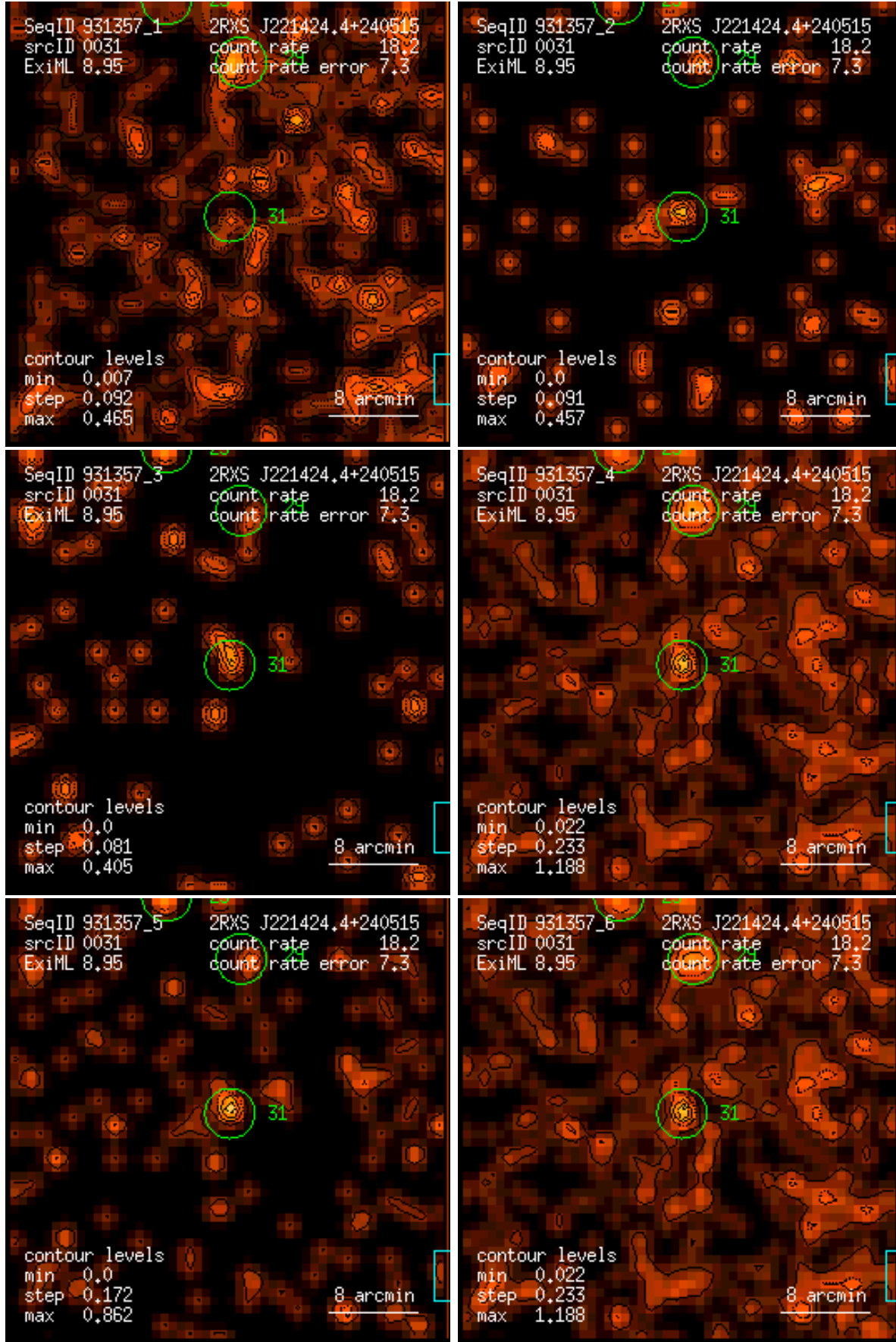
Figure 31: RASS 931357: detection 0031: band rate images, Gaussian filter: (1) PSPC channels 11 – 41, (2) 52 – 90, (3) 91 – 201, (4) 11 – 235, (5) 52 – 201, (6) 11 – 201. Broad band rates in counts/ks. Band rate contour levels in counts/ks/arcmin 2 .
