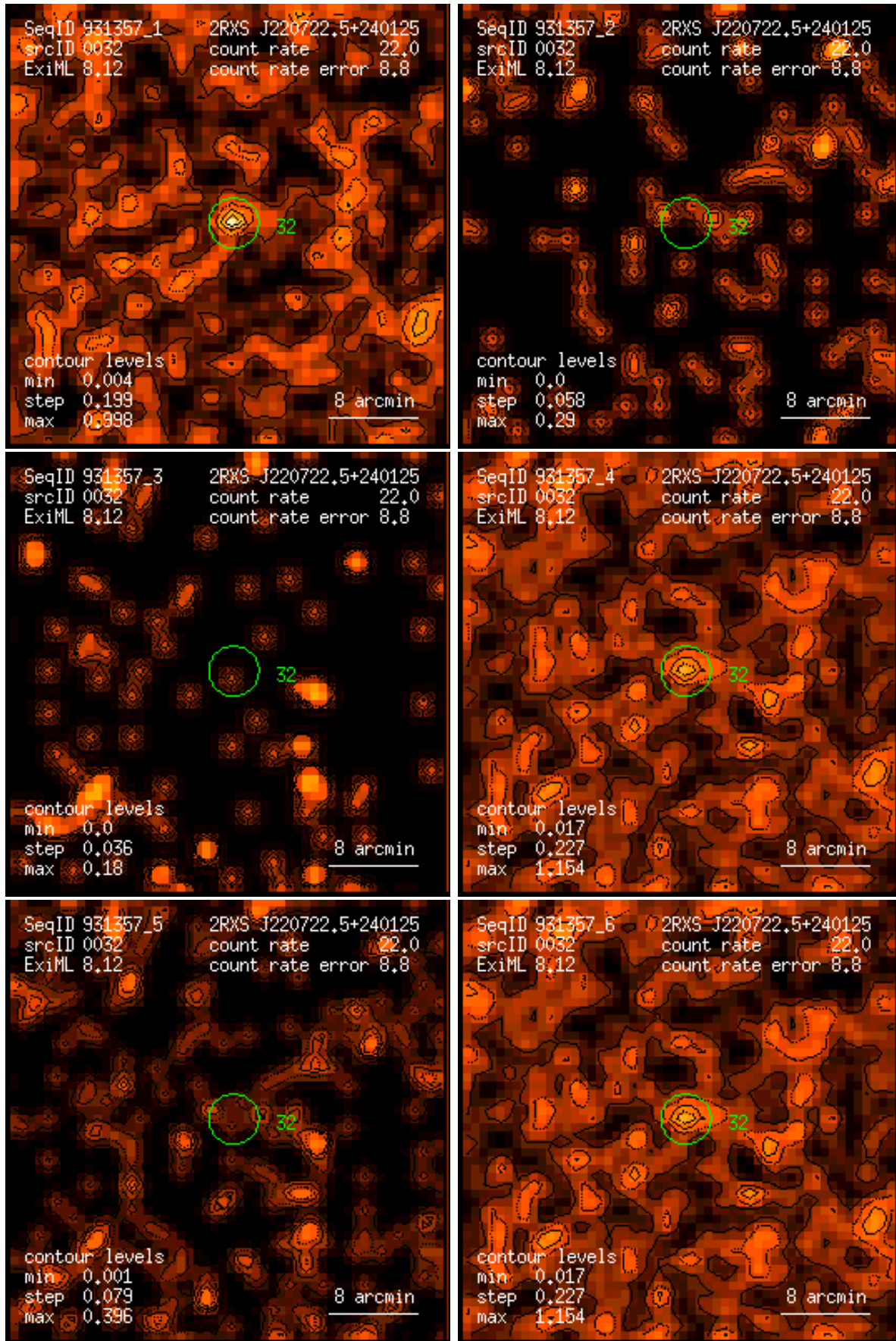
Figure 32: RASS 931357: detection 0032: band rate images, Gaussian filter: (1) PSPC channels 11 – 41, (2) 52 – 90, (3) 91 – 201, (4) 11 – 235, (5) 52 – 201, (6) 11 – 201. Broad band rates in counts/ks. Band rate contour levels in counts/ks/arcmin 2 .
