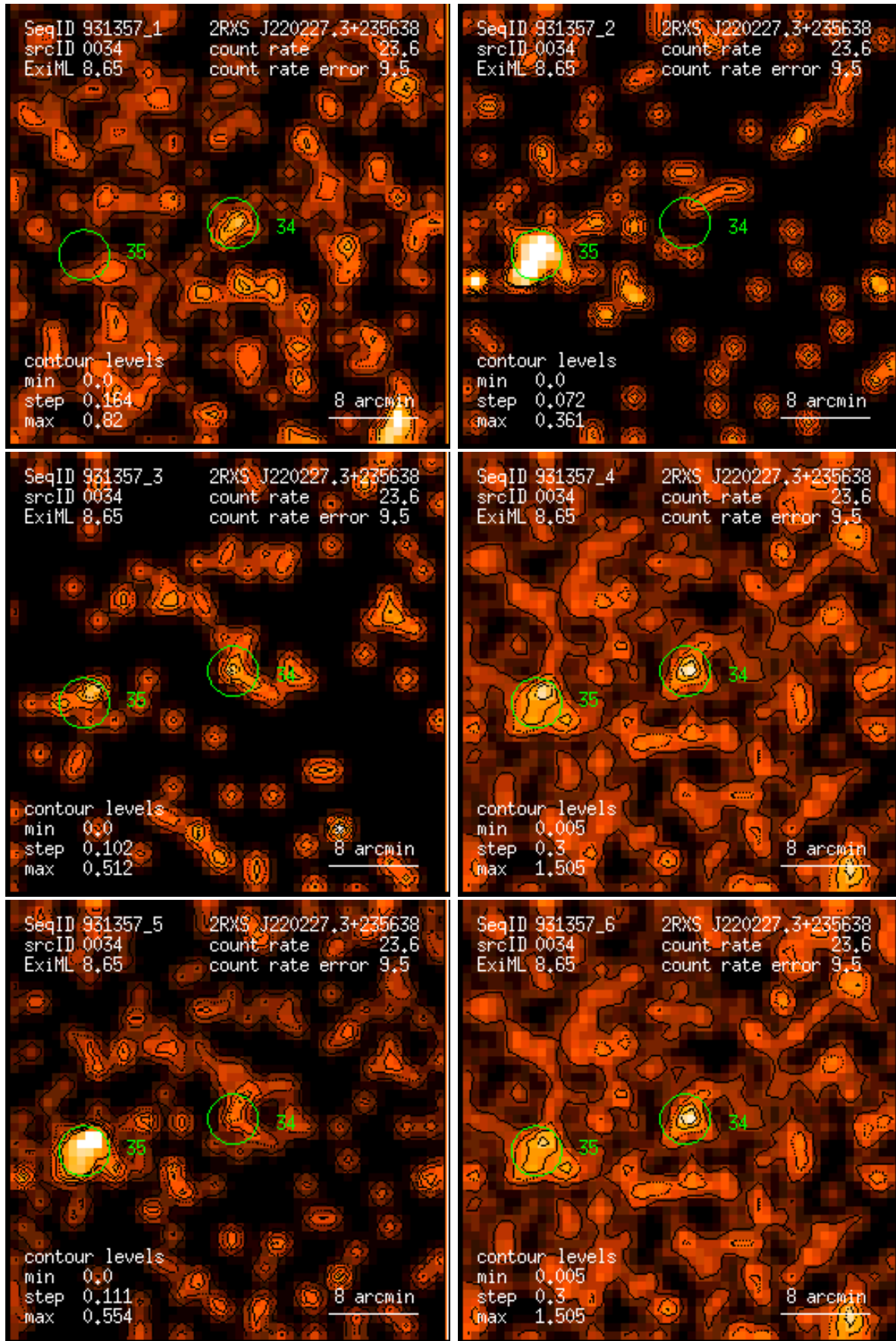
Figure 34: RASS 931357: detection 0034: band rate images, Gaussian filter: (1) PSPC channels 11 – 41, (2) 52 – 90, (3) 91 – 201, (4) 11 – 235, (5) 52 – 201, (6) 11 – 201. Broad band rates in counts/ks. Band rate contour levels in counts/ks/arcmin 2 .
