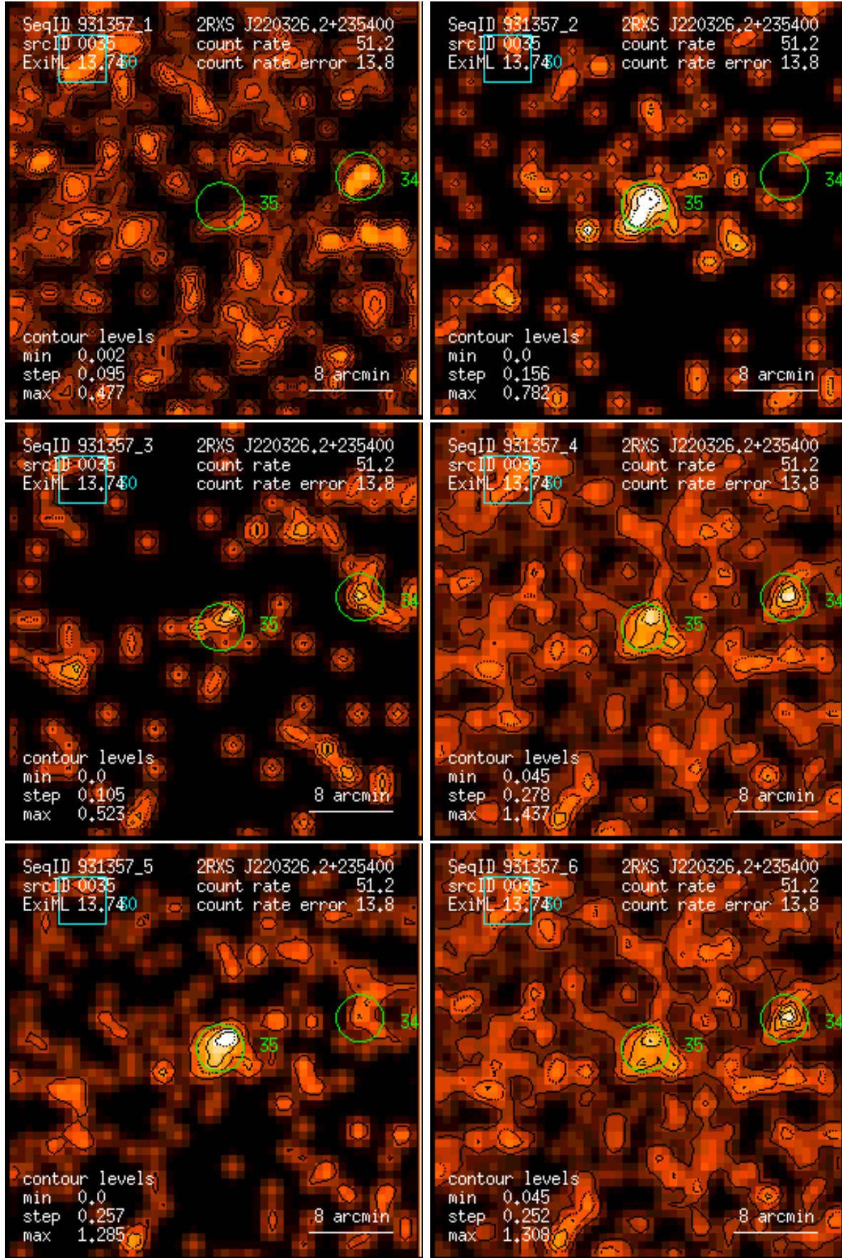
Figure 35: RASS 931357: detection 0035: band rate images, Gaussian filter: (1) PSPC channels 11 – 41, (2) 52 – 90, (3) 91 – 201, (4) 11 – 235, (5) 52 – 201, (6) 11 – 201. Broad band rates in counts/ks. Band rate contour levels in counts/ks/arcmin 2 .
