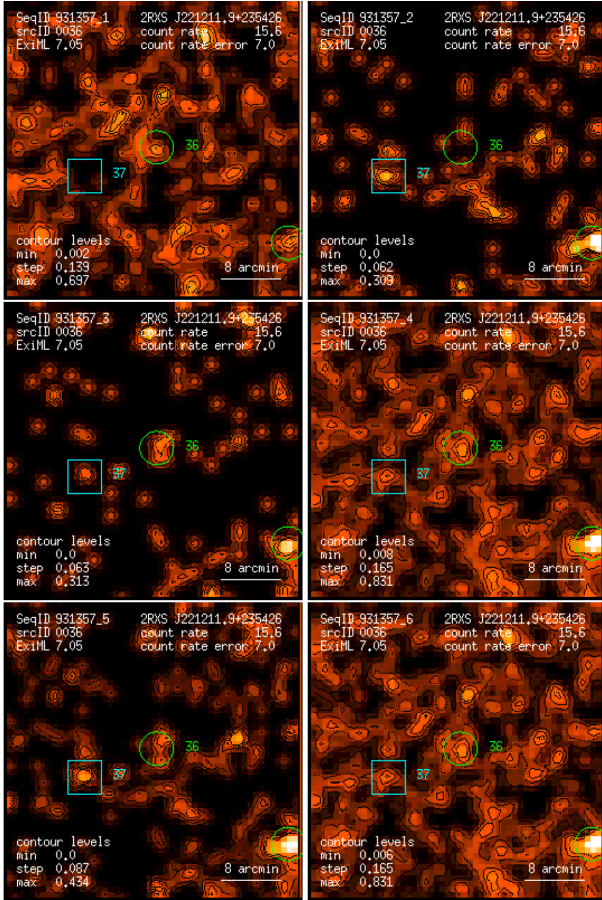
Figure 36: RASS 931357: detection 0036: band rate images, Gaussian filter: (1) PSPC channels 11 – 41, (2) 52 – 90, (3) 91 – 201, (4) 11 – 235, (5) 52 – 201, (6) 11 – 201. Broad band rates in counts/ks. Band rate contour levels in counts/ks/arcmin 2 .
