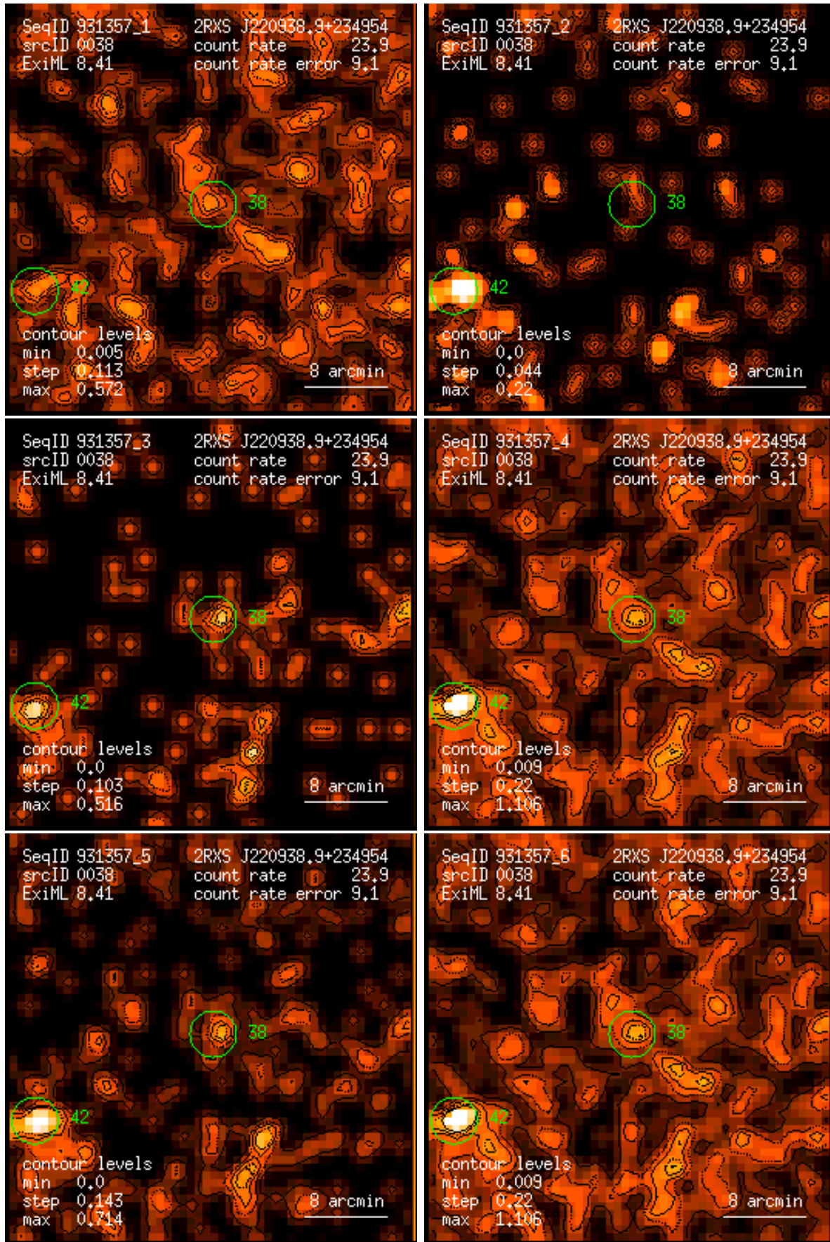
Figure 38: RASS 931357: detection 0038: band rate images, Gaussian filter: (1) PSPC channels 11 – 41, (2) 52 – 90, (3) 91 – 201, (4) 11 – 235, (5) 52 – 201, (6) 11 – 201. Broad band rates in counts/ks. Band rate contour levels in counts/ks/arcmin 2 .
