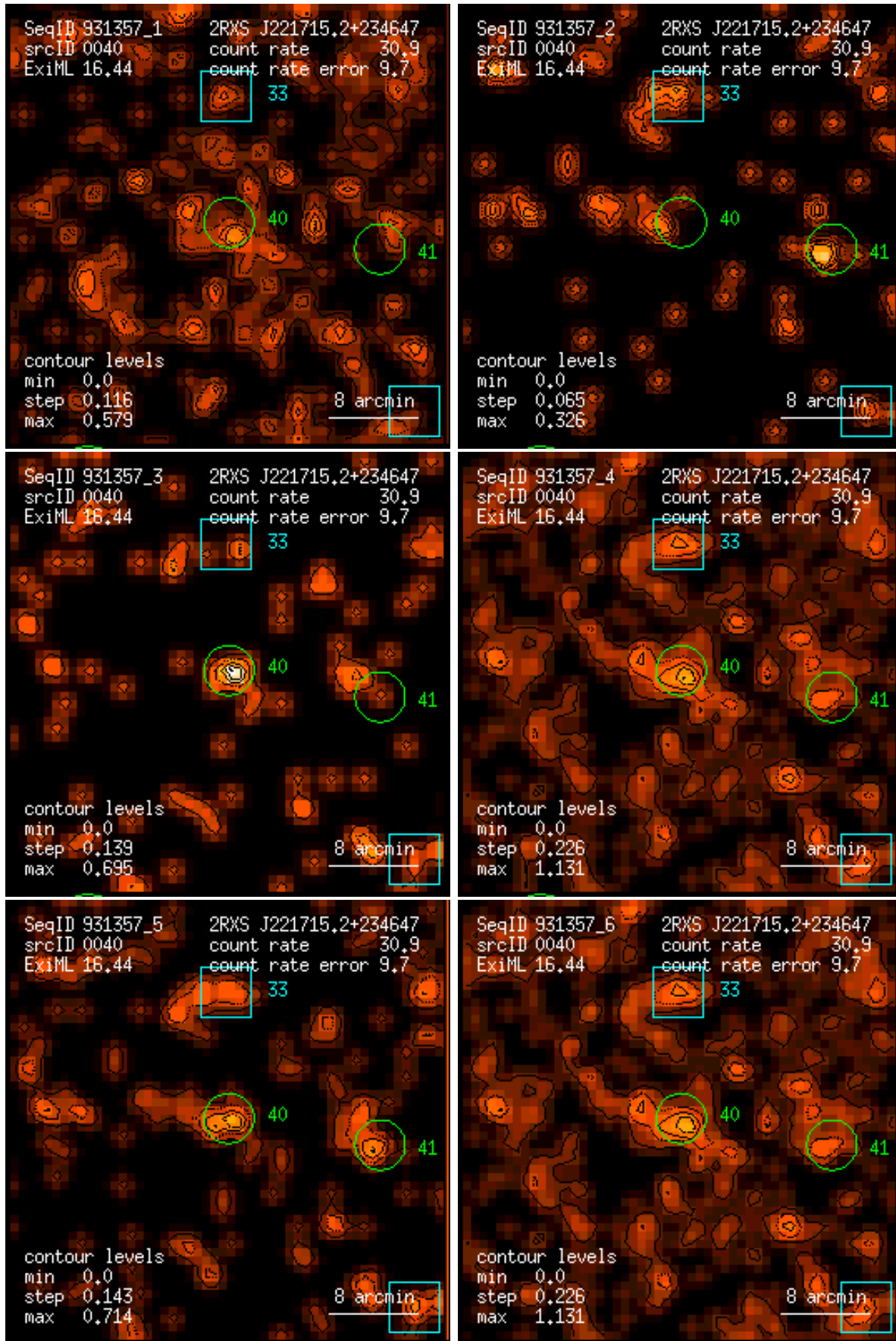
Figure 40: RASS 931357: detection 0040: band rate images, Gaussian filter: (1) PSPC channels 11 – 41, (2) 52 – 90, (3) 91 – 201, (4) 11 – 235, (5) 52 – 201, (6) 11 – 201. Broad band rates in counts/ks. Band rate contour levels in counts/ks/arcmin 2 .
