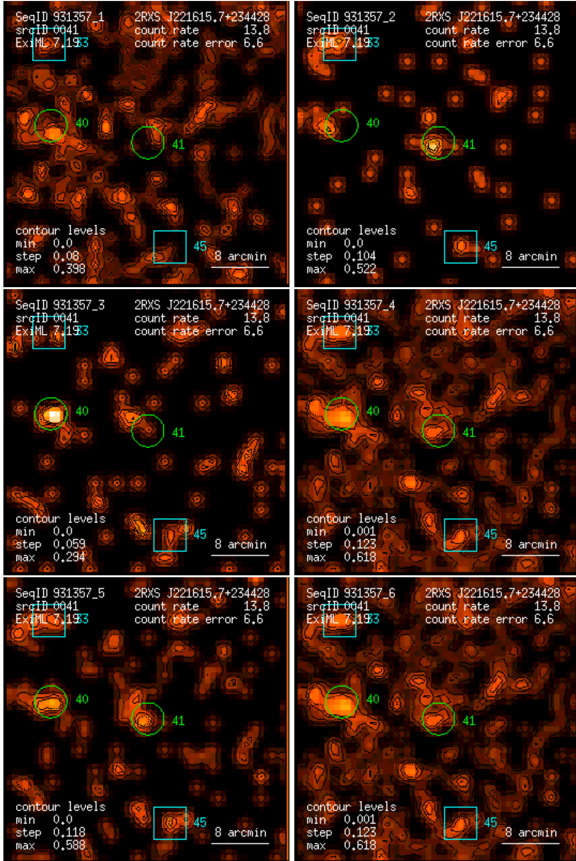
Figure 41: RASS 931357: detection 0041: band rate images, Gaussian filter: (1) PSPC channels 11 – 41, (2) 52 – 90, (3) 91 – 201, (4) 11 – 235, (5) 52 – 201, (6) 11 – 201. Broad band rates in counts/ks. Band rate contour levels in counts/ks/arcmin 2 .
