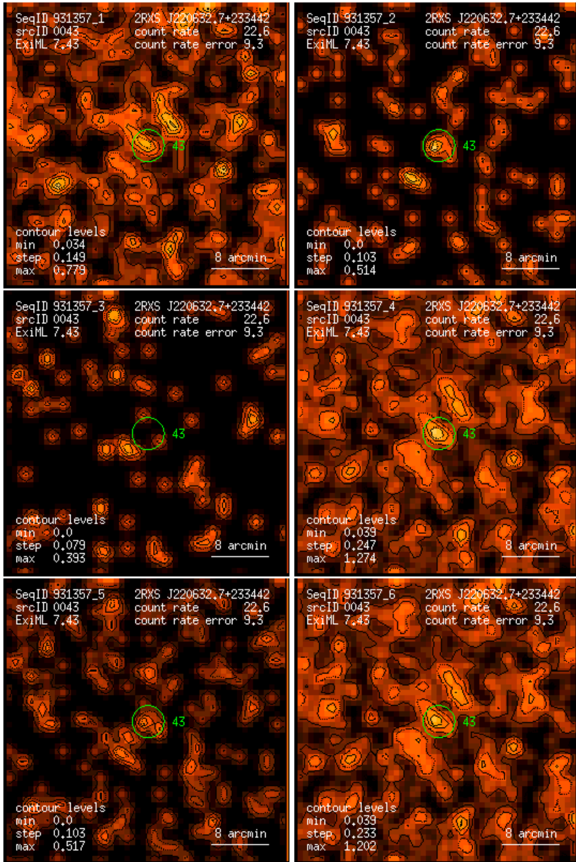
Figure 43: RASS 931357: detection 0043: band rate images, Gaussian filter: (1) PSPC channels 11 – 41, (2) 52 – 90, (3) 91 – 201, (4) 11 – 235, (5) 52 – 201, (6) 11 – 201. Broad band rates in counts/ks. Band rate contour levels in counts/ks/arcmin 2 .
