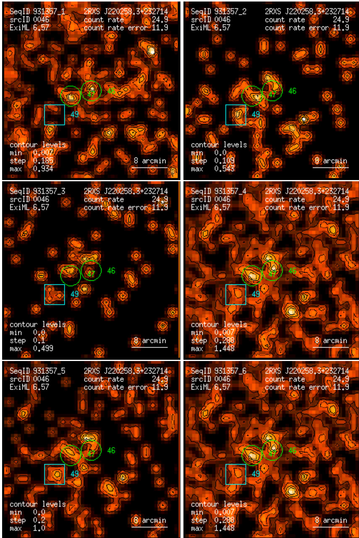
Figure 46: RASS 931357: detection 0046: band rate images, Gaussian filter: (1) PSPC channels 11 – 41, (2) 52 – 90, (3) 91 – 201, (4) 11 – 235, (5) 52 – 201, (6) 11 – 201. Broad band rates in counts/ks. Band rate contour levels in counts/ks/arcmin 2 .
