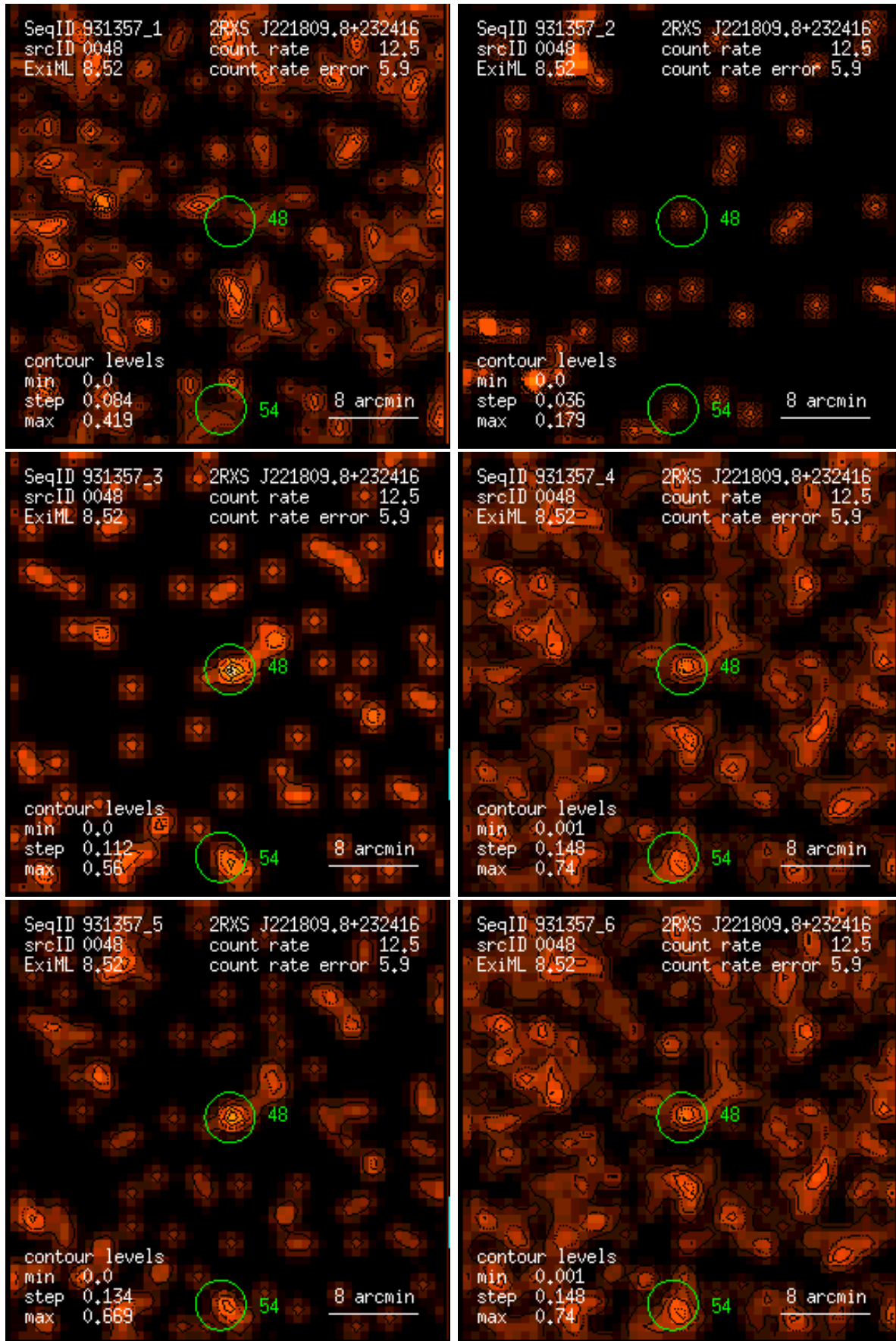
Figure 48: RASS 931357: detection 0048: band rate images, Gaussian filter: (1) PSPC channels 11 – 41, (2) 52 – 90, (3) 91 – 201, (4) 11 – 235, (5) 52 – 201, (6) 11 – 201. Broad band rates in counts/ks. Band rate contour levels in counts/ks/arcmin 2 .
