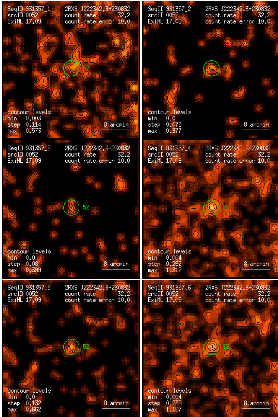
Figure 52: RASS 931357: detection 0052: band rate images, Gaussian filter: (1) PSPC channels 11 – 41, (2) 52 – 90, (3) 91 – 201, (4) 11 – 235, (5) 52 – 201, (6) 11 – 201. Broad band rates in counts/ks. Band rate contour levels in counts/ks/arcmin 2 .
