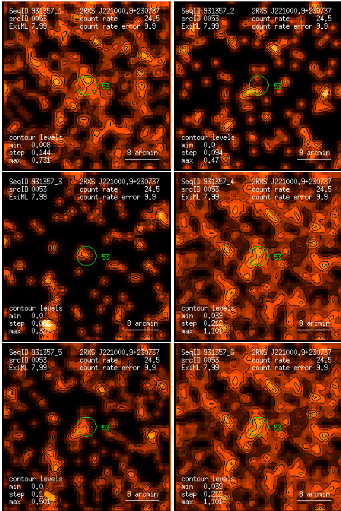
Figure 53: RASS 931357: detection 0053: band rate images, Gaussian filter: (1) PSPC channels 11 – 41, (2) 52 – 90, (3) 91 – 201, (4) 11 – 235, (5) 52 – 201, (6) 11 – 201. Broad band rates in counts/ks. Band rate contour levels in counts/ks/arcmin 2 .
