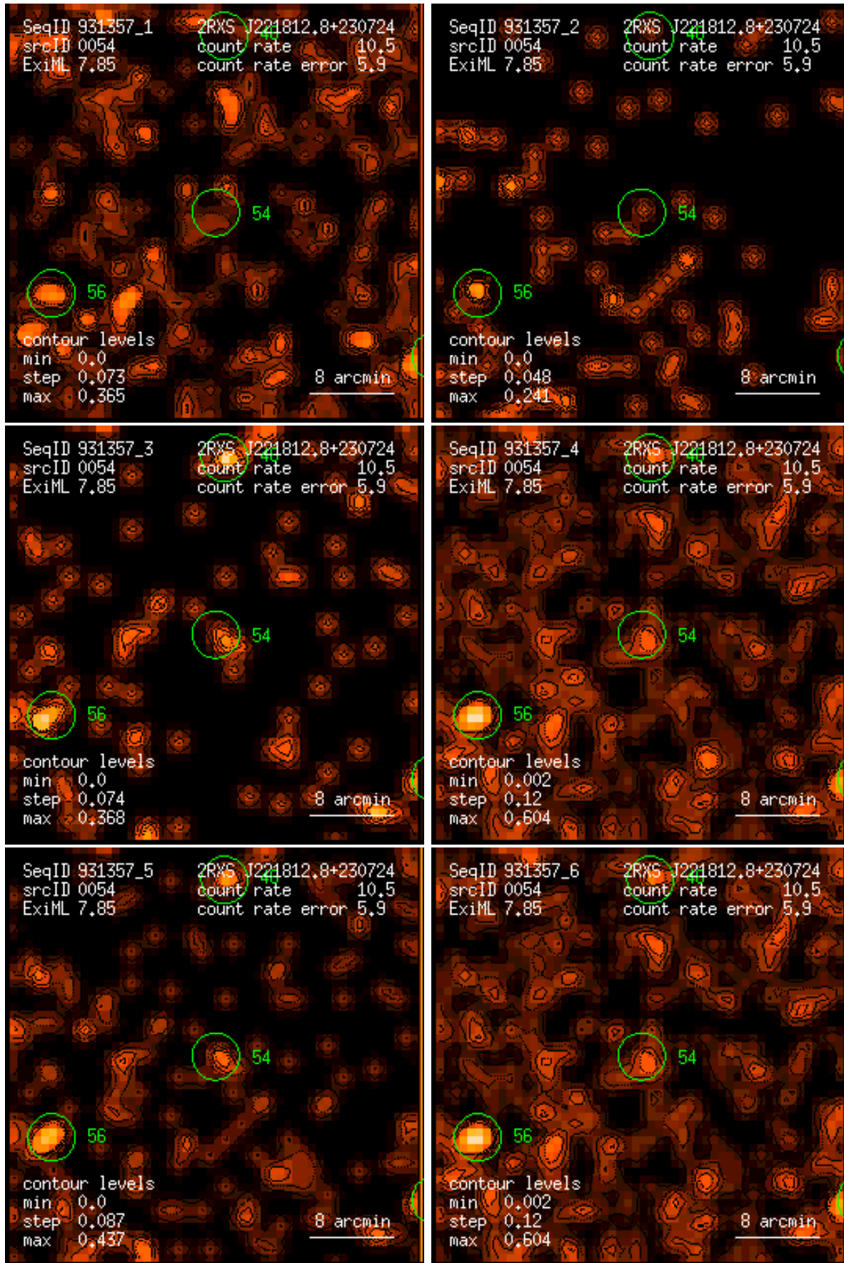
Figure 54: RASS 931357: detection 0054: band rate images, Gaussian filter: (1) PSPC channels 11 – 41, (2) 52 – 90, (3) 91 – 201, (4) 11 – 235, (5) 52 – 201, (6) 11 – 201. Broad band rates in counts/ks. Band rate contour levels in counts/ks/arcmin 2 .
