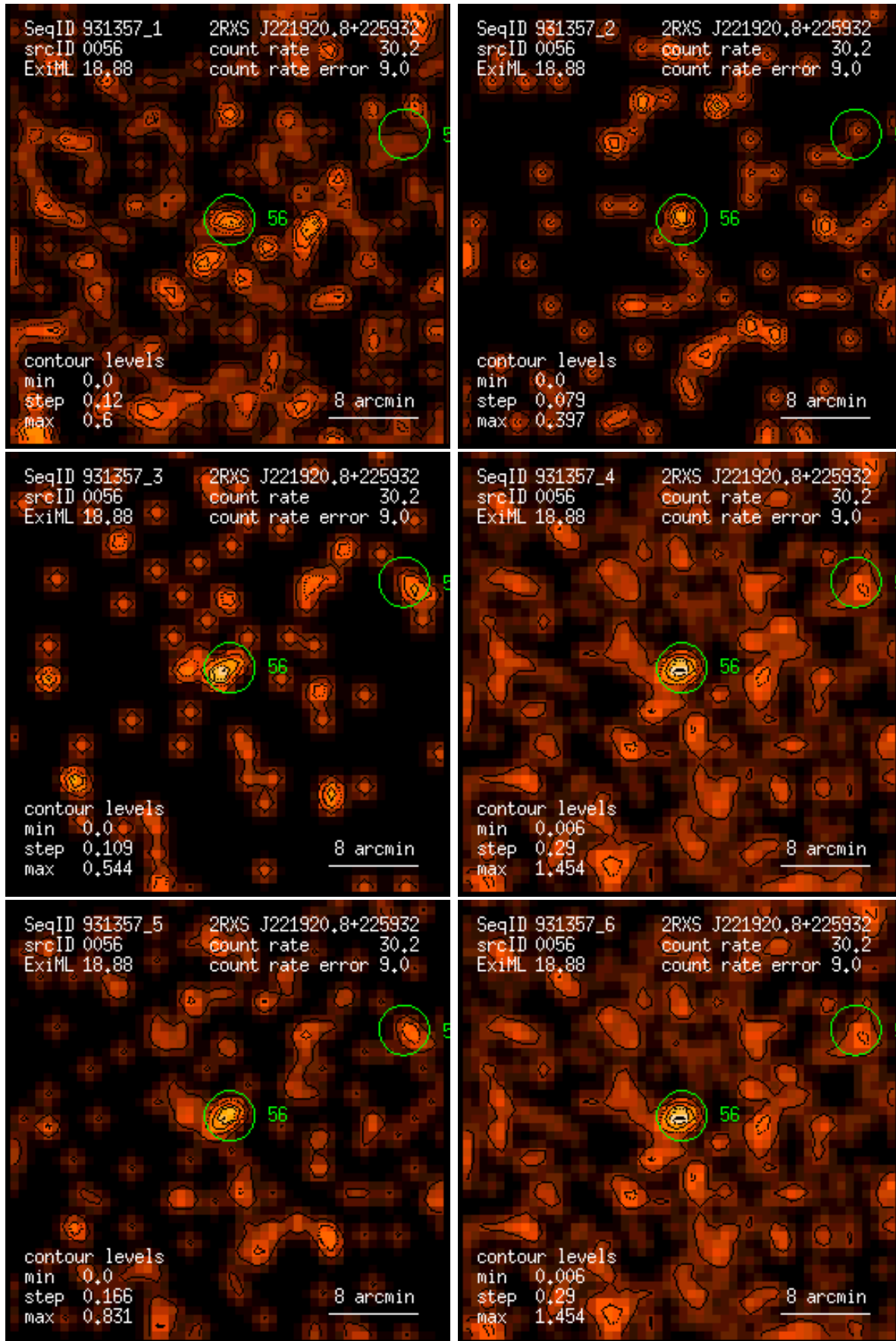
Figure 56: RASS 931357: detection 0056: band rate images, Gaussian filter: (1) PSPC channels 11 – 41, (2) 52 – 90, (3) 91 – 201, (4) 11 – 235, (5) 52 – 201, (6) 11 – 201. Broad band rates in counts/ks. Band rate contour levels in counts/ks/arcmin 2 .
