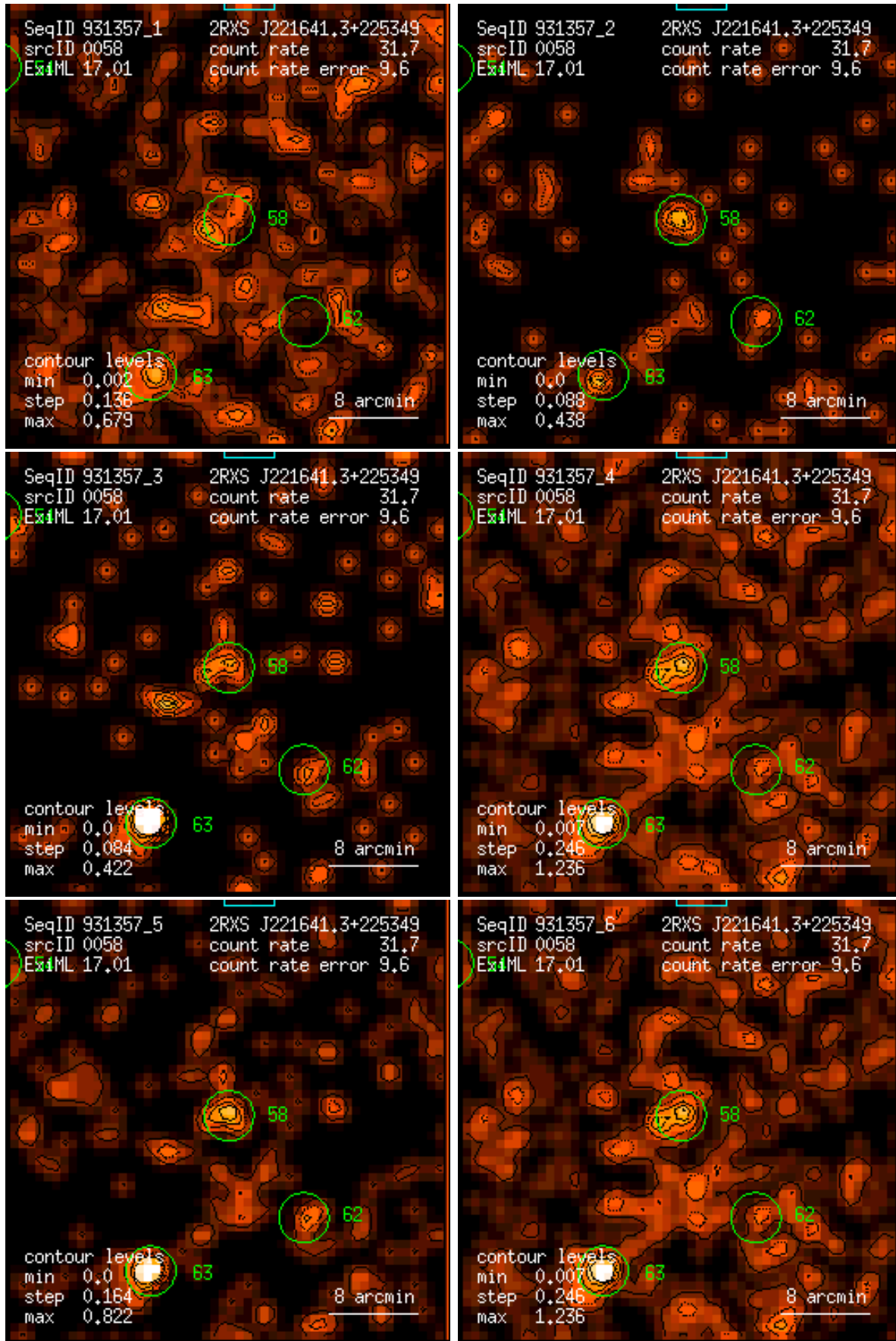
Figure 58: RASS 931357: detection 0058: band rate images, Gaussian filter: (1) PSPC channels 11 – 41, (2) 52 – 90, (3) 91 – 201, (4) 11 – 235, (5) 52 – 201, (6) 11 – 201. Broad band rates in counts/ks. Band rate contour levels in counts/ks/arcmin 2 .
