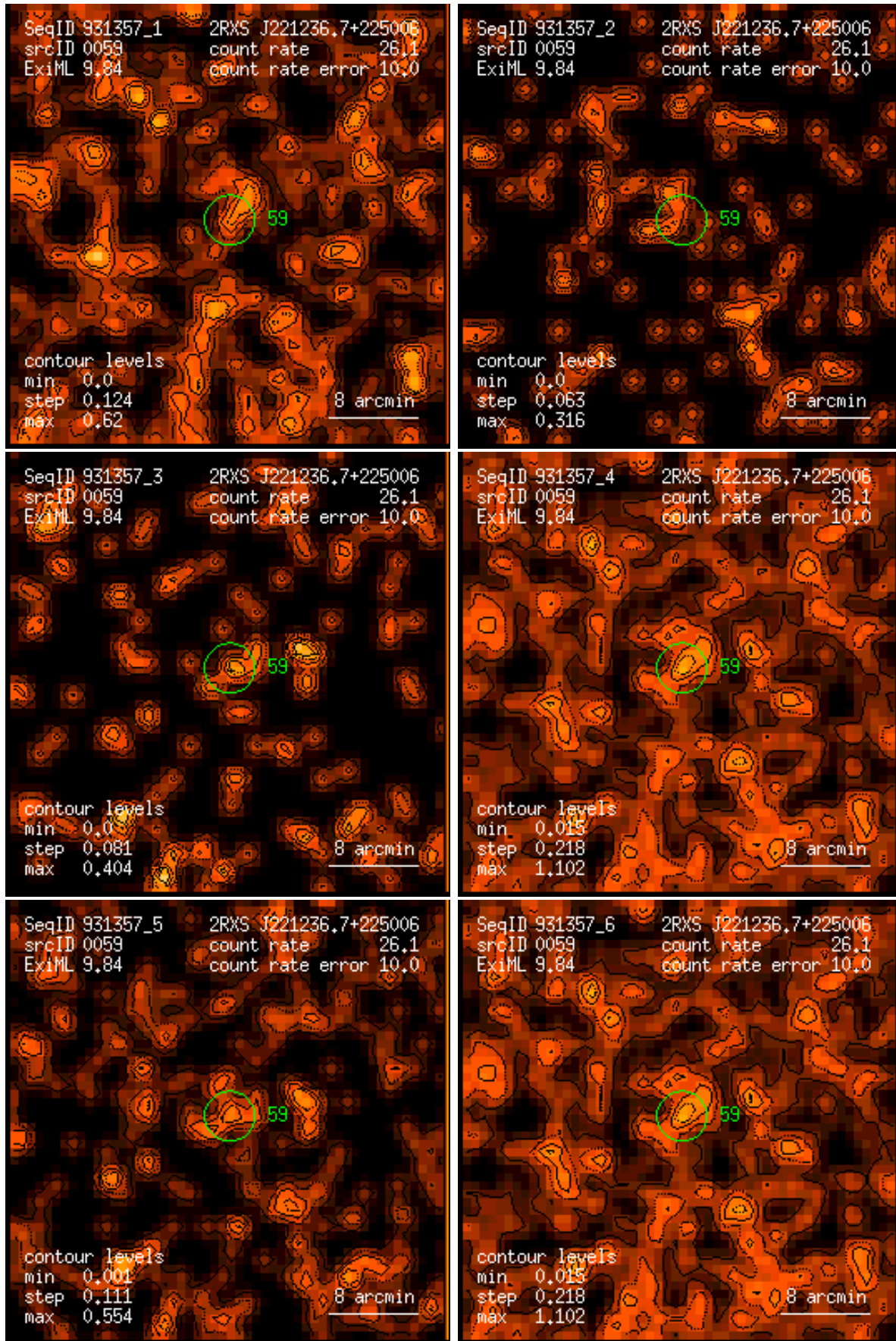
Figure 59: RASS 931357: detection 0059: band rate images, Gaussian filter: (1) PSPC channels 11 – 41, (2) 52 – 90, (3) 91 – 201, (4) 11 – 235, (5) 52 – 201, (6) 11 – 201. Broad band rates in counts/ks. Band rate contour levels in counts/ks/arcmin 2 .
