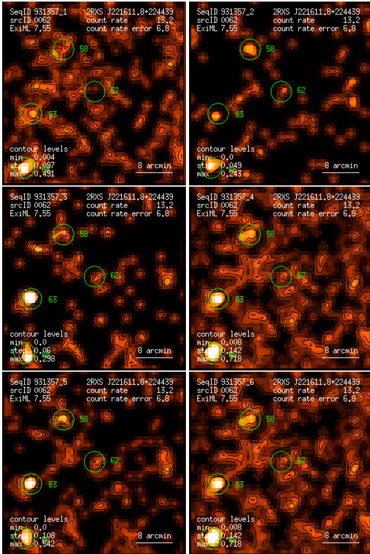
Figure 62: RASS 931357: detection 0062: band rate images, Gaussian filter: (1) PSPC channels 11 – 41, (2) 52 – 90, (3) 91 – 201, (4) 11 – 235, (5) 52 – 201, (6) 11 – 201. Broad band rates in counts/ks. Band rate contour levels in counts/ks/arcmin 2 .
