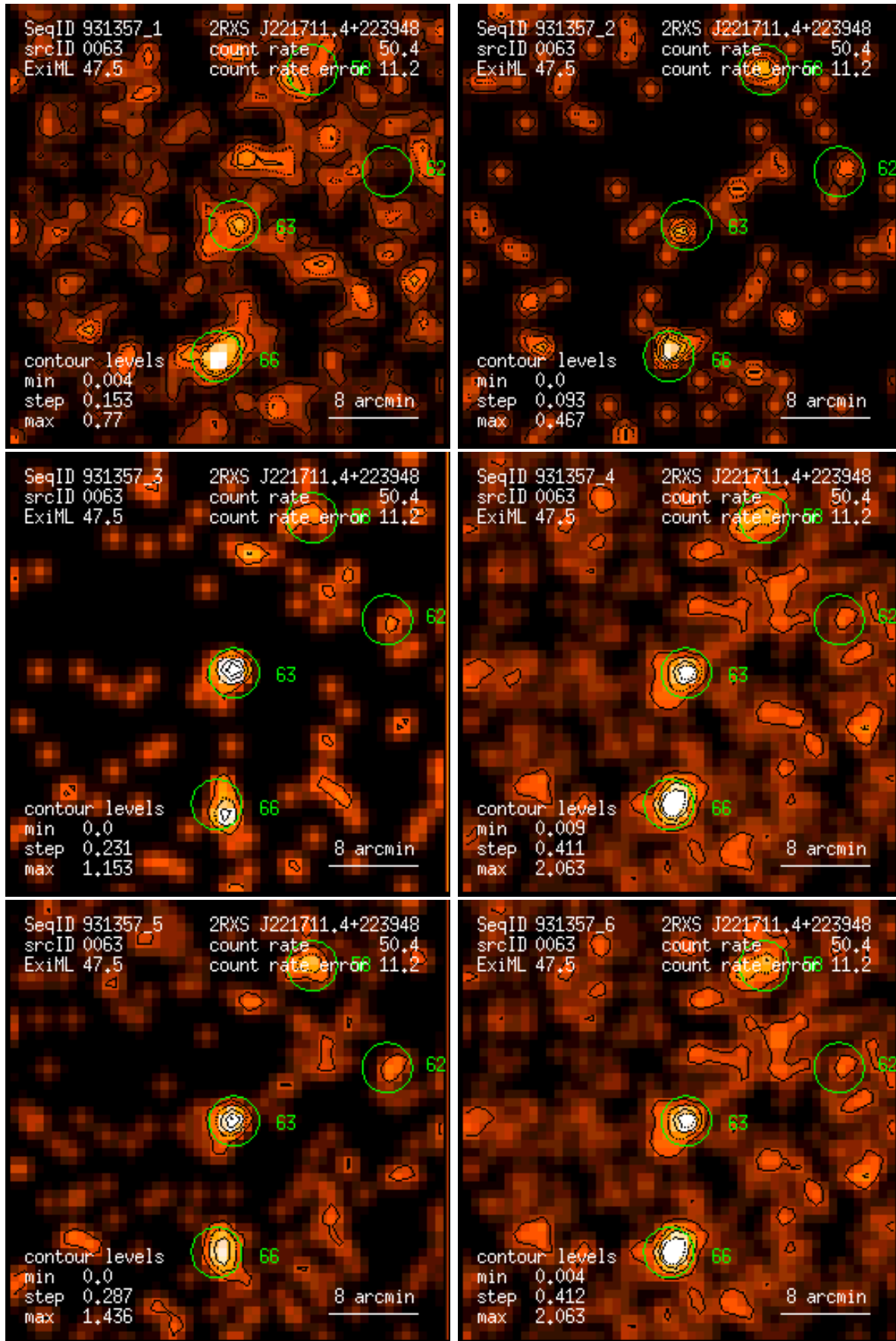
Figure 63: RASS 931357: detection 0063: band rate images, Gaussian filter: (1) PSPC channels 11 – 41, (2) 52 – 90, (3) 91 – 201, (4) 11 – 235, (5) 52 – 201, (6) 11 – 201. Broad band rates in counts/ks. Band rate contour levels in counts/ks/arcmin 2 .
