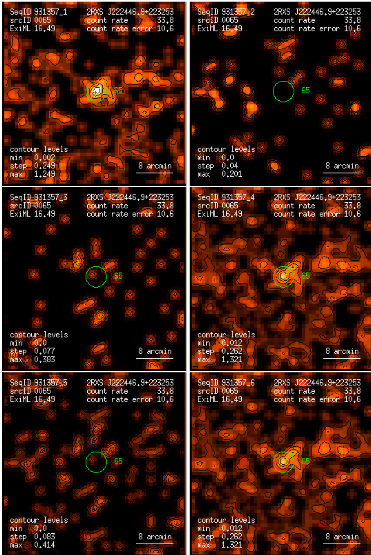
Figure 65: RASS 931357: detection 0065: band rate images, Gaussian filter: (1) PSPC channels 11 – 41, (2) 52 – 90, (3) 91 – 201, (4) 11 – 235, (5) 52 – 201, (6) 11 – 201. Broad band rates in counts/ks. Band rate contour levels in counts/ks/arcmin 2 .
