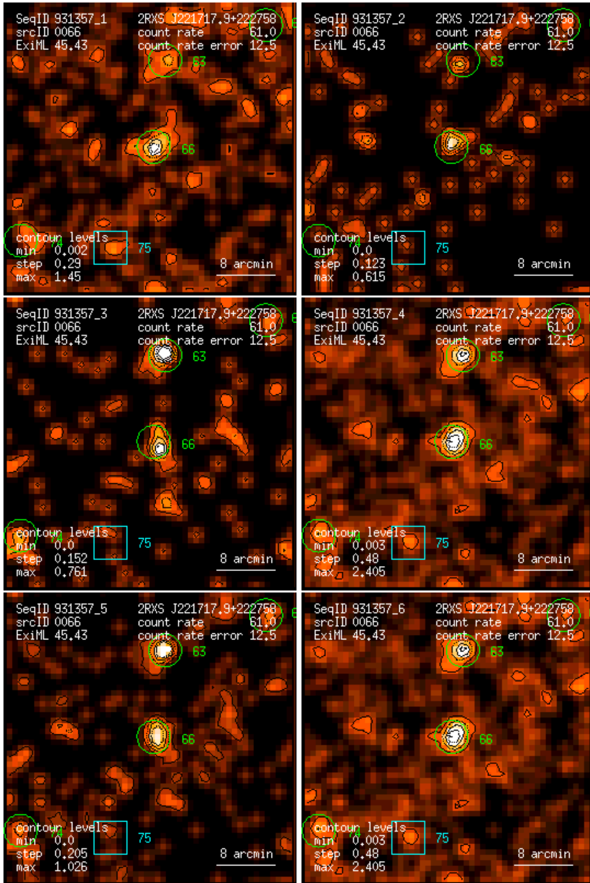
Figure 66: RASS 931357: detection 0066: band rate images, Gaussian filter: (1) PSPC channels 11 – 41, (2) 52 – 90, (3) 91 – 201, (4) 11 – 235, (5) 52 – 201, (6) 11 – 201. Broad band rates in counts/ks. Band rate contour levels in counts/ks/arcmin 2 .
