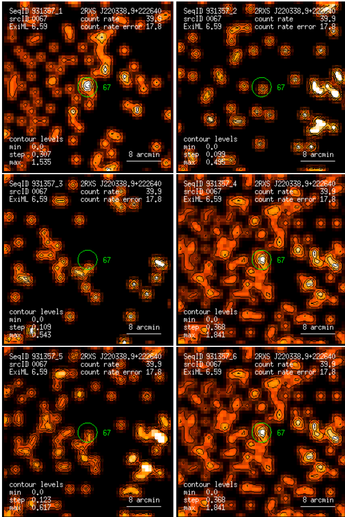
Figure 67: RASS 931357: detection 0067: band rate images, Gaussian filter: (1) PSPC channels 11 – 41, (2) 52 – 90, (3) 91 – 201, (4) 11 – 235, (5) 52 – 201, (6) 11 – 201. Broad band rates in counts/ks. Band rate contour levels in counts/ks/arcmin 2 .
