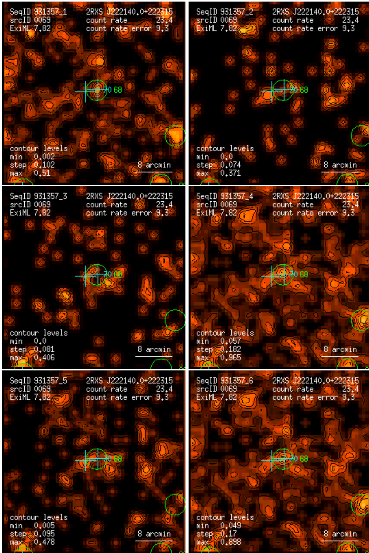
Figure 69: RASS 931357: detection 0069: band rate images, Gaussian filter: (1) PSPC channels 11 – 41, (2) 52 – 90, (3) 91 – 201, (4) 11 – 235, (5) 52 – 201, (6) 11 – 201. Broad band rates in counts/ks. Band rate contour levels in counts/ks/arcmin 2 .
