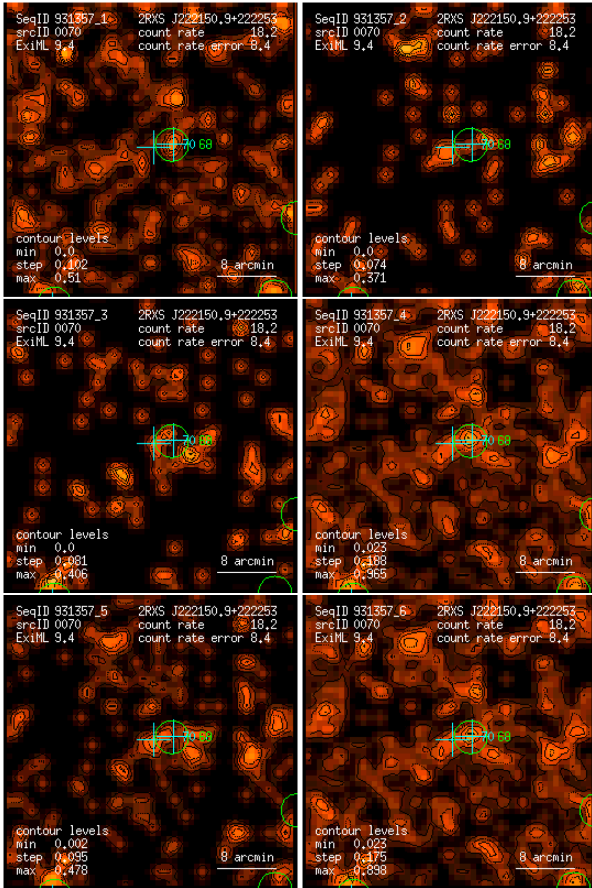
Figure 70: RASS 931357: detection 0070: band rate images, Gaussian filter: (1) PSPC channels 11 – 41, (2) 52 – 90, (3) 91 – 201, (4) 11 – 235, (5) 52 – 201, (6) 11 – 201. Broad band rates in counts/ks. Band rate contour levels in counts/ks/arcmin 2 .
