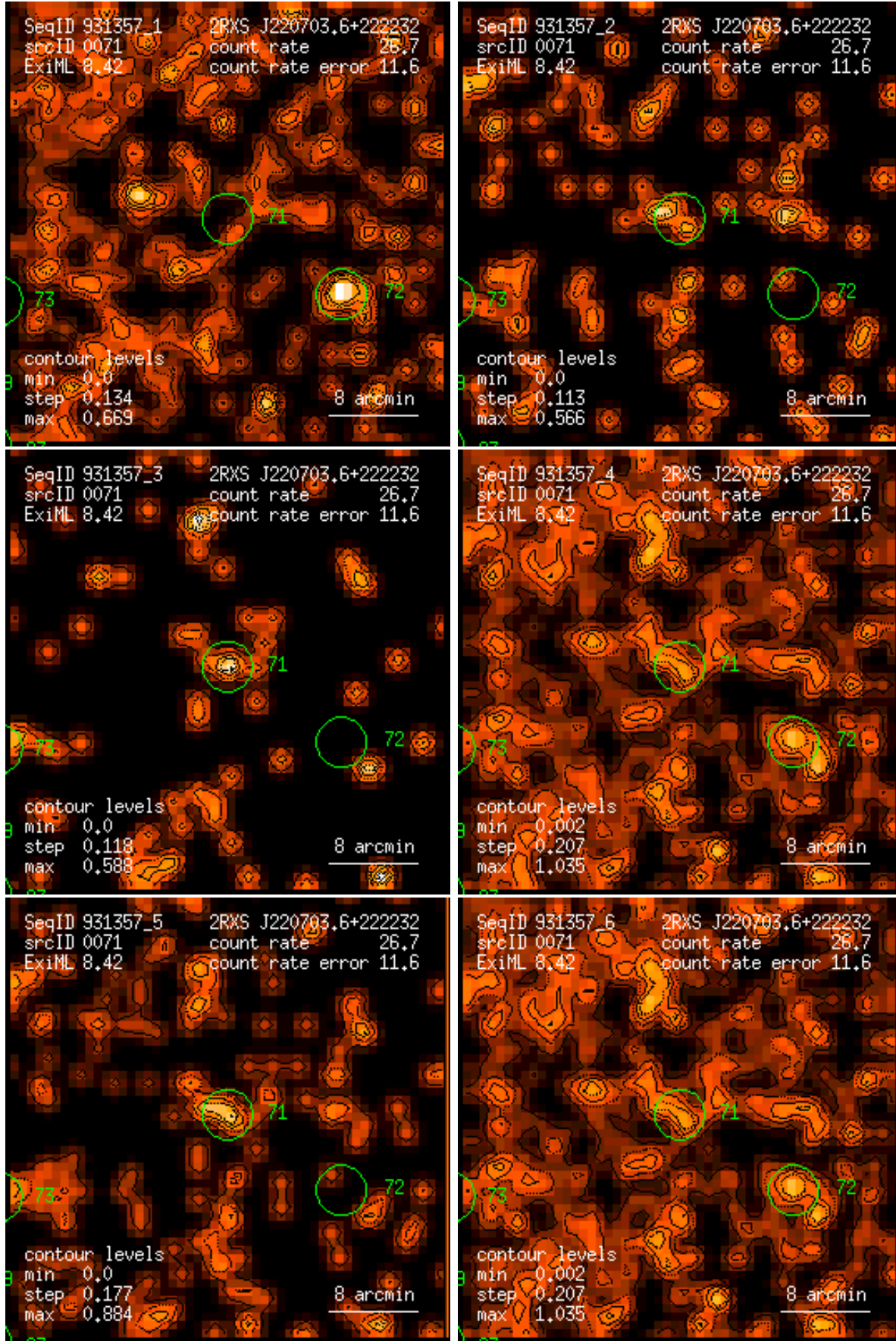
Figure 71: RASS 931357: detection 0071: band rate images, Gaussian filter: (1) PSPC channels 11 – 41, (2) 52 – 90, (3) 91 – 201, (4) 11 – 235, (5) 52 – 201, (6) 11 – 201. Broad band rates in counts/ks. Band rate contour levels in counts/ks/arcmin 2 .
