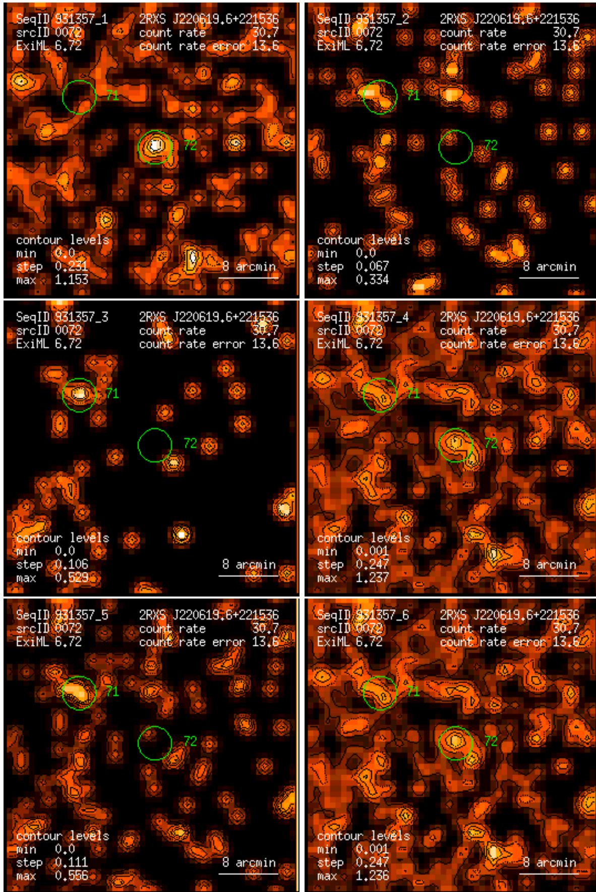
Figure 72: RASS 931357: detection 0072: band rate images, Gaussian filter: (1) PSPC channels 11 – 41, (2) 52 – 90, (3) 91 – 201, (4) 11 – 235, (5) 52 – 201, (6) 11 – 201. Broad band rates in counts/ks. Band rate contour levels in counts/ks/arcmin 2 .
