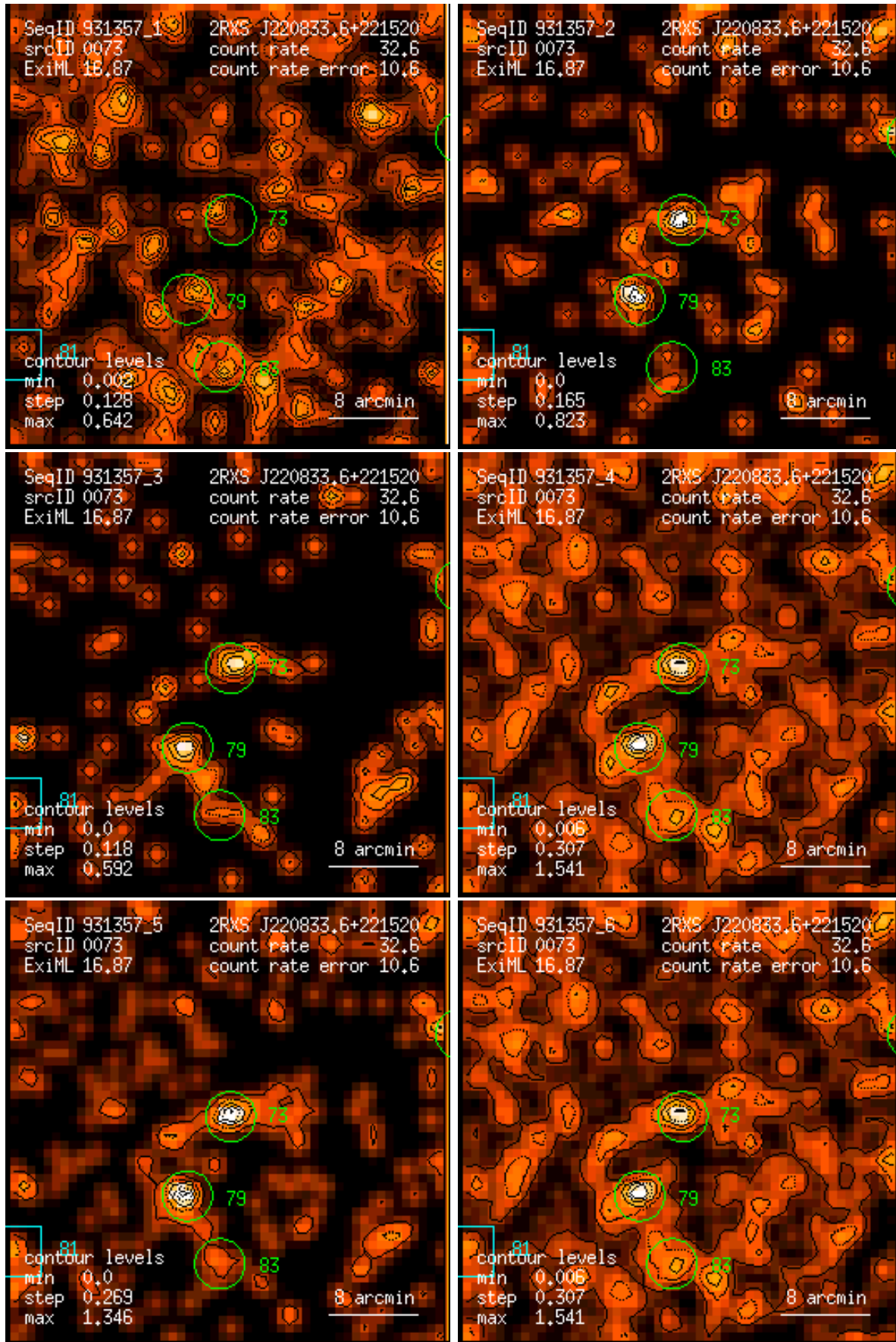
Figure 73: RASS 931357: detection 0073: band rate images, Gaussian filter: (1) PSPC channels 11 – 41, (2) 52 – 90, (3) 91 – 201, (4) 11 – 235, (5) 52 – 201, (6) 11 – 201. Broad band rates in counts/ks. Band rate contour levels in counts/ks/arcmin 2 .
