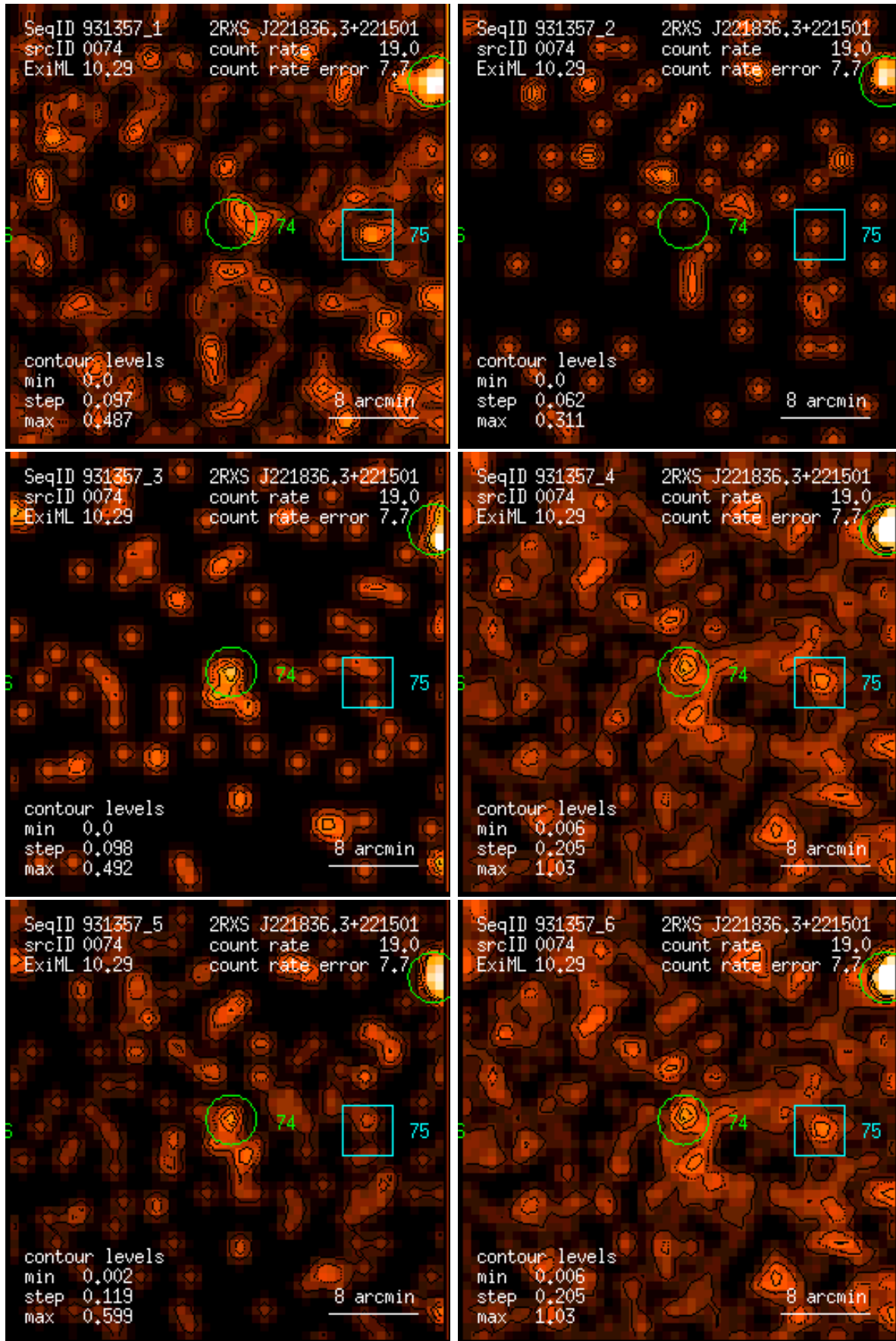
Figure 74: RASS 931357: detection 0074: band rate images, Gaussian filter: (1) PSPC channels 11 – 41, (2) 52 – 90, (3) 91 – 201, (4) 11 – 235, (5) 52 – 201, (6) 11 – 201. Broad band rates in counts/ks. Band rate contour levels in counts/ks/arcmin 2 .
