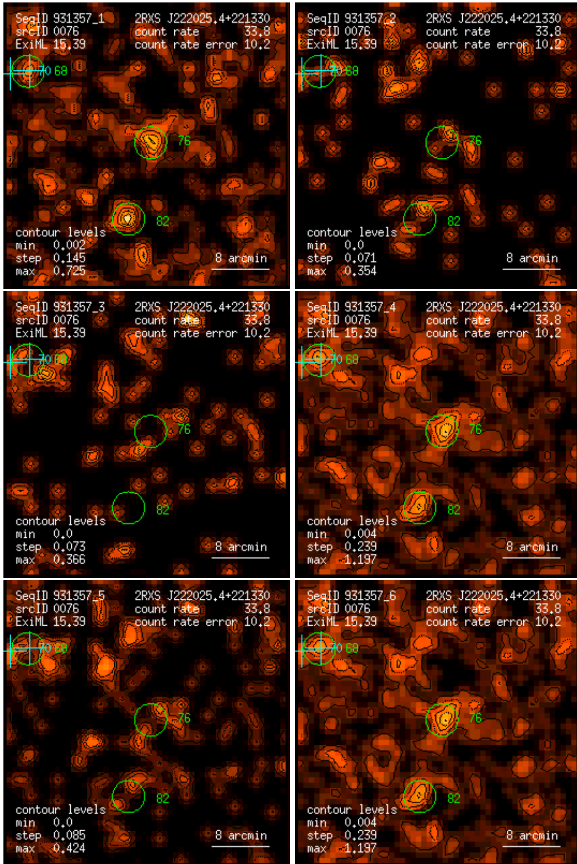
Figure 76: RASS 931357: detection 0076: band rate images, Gaussian filter: (1) PSPC channels 11 – 41, (2) 52 – 90, (3) 91 – 201, (4) 11 – 235, (5) 52 – 201, (6) 11 – 201. Broad band rates in counts/ks. Band rate contour levels in counts/ks/arcmin 2 .
