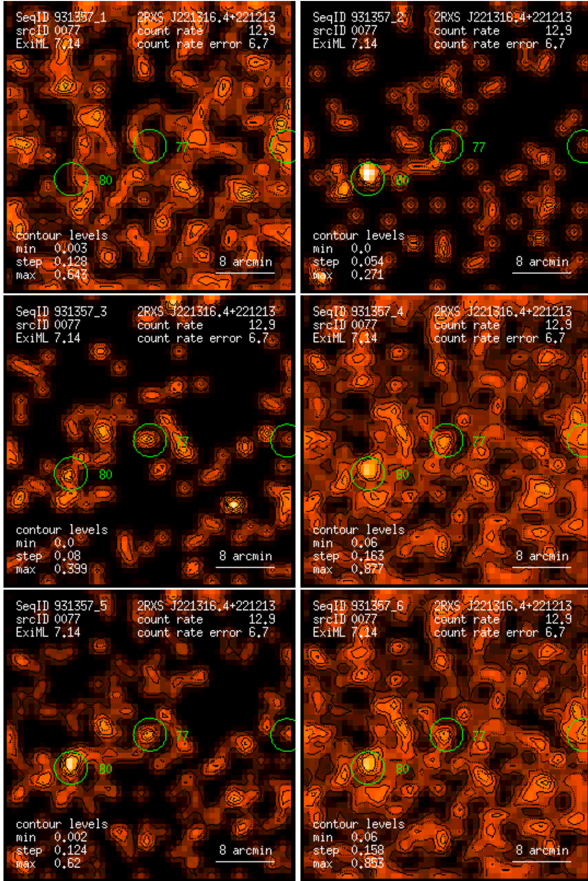
Figure 77: RASS 931357: detection 0077: band rate images, Gaussian filter: (1) PSPC channels 11 – 41, (2) 52 – 90, (3) 91 – 201, (4) 11 – 235, (5) 52 – 201, (6) 11 – 201. Broad band rates in counts/ks. Band rate contour levels in counts/ks/arcmin 2 .
