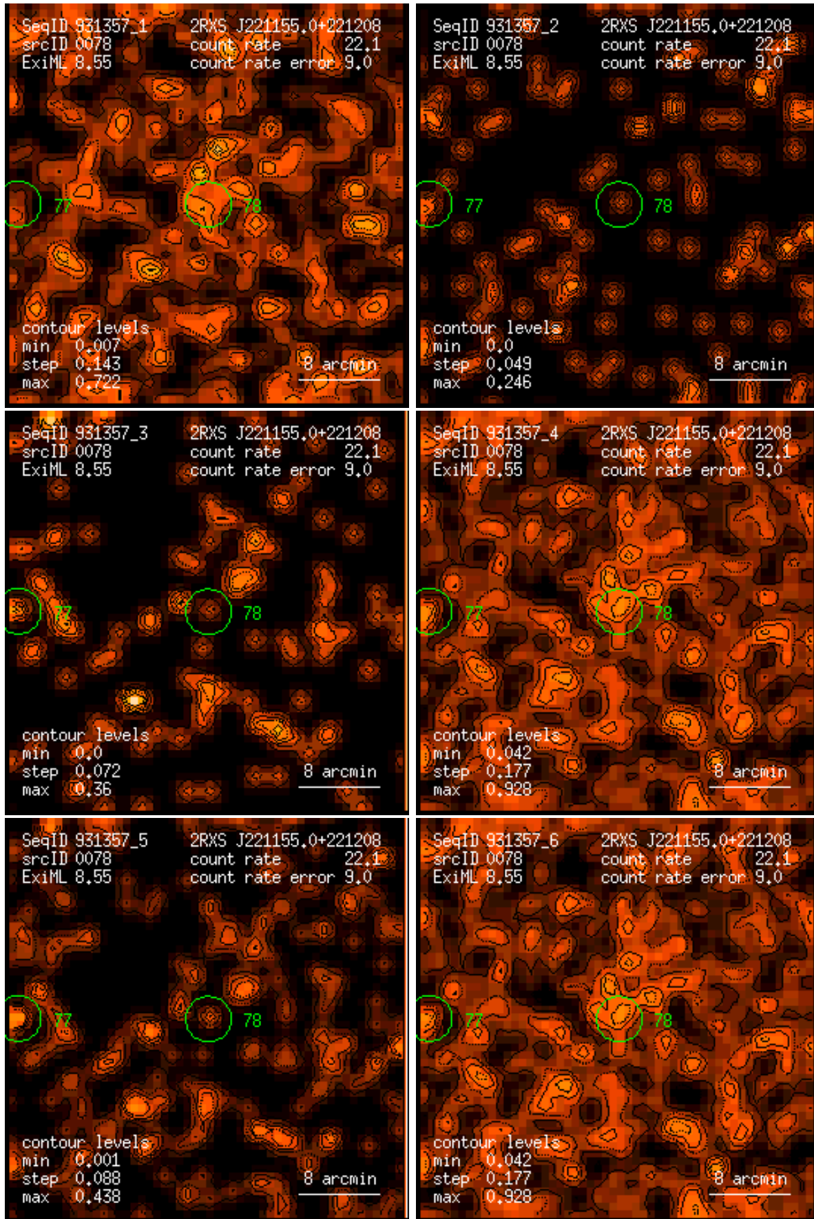
Figure 78: RASS 931357: detection 0078: band rate images, Gaussian filter: (1) PSPC channels 11 – 41, (2) 52 – 90, (3) 91 – 201, (4) 11 – 235, (5) 52 – 201, (6) 11 – 201. Broad band rates in counts/ks. Band rate contour levels in counts/ks/arcmin 2 .
