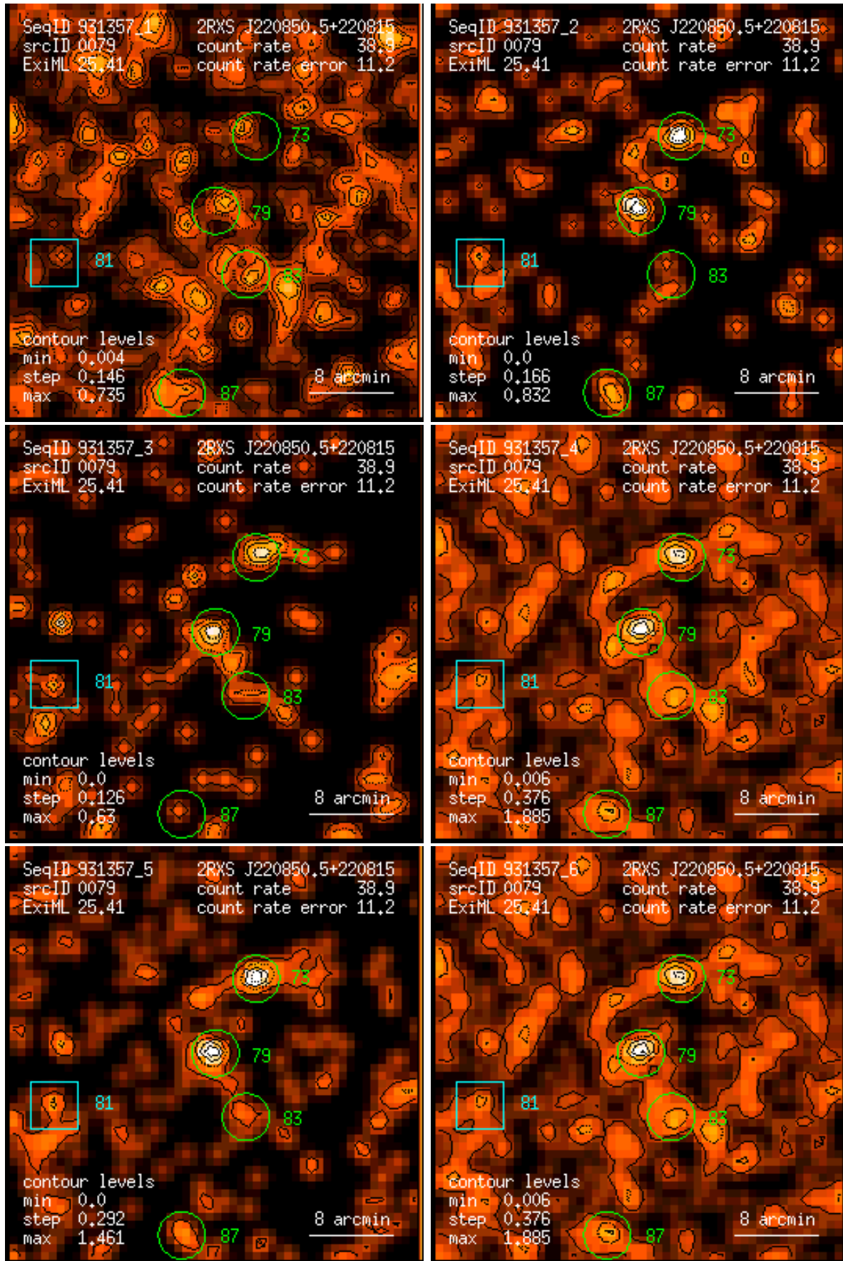
Figure 79: RASS 931357: detection 0079: band rate images, Gaussian filter: (1) PSPC channels 11 – 41, (2) 52 – 90, (3) 91 – 201, (4) 11 – 235, (5) 52 – 201, (6) 11 – 201. Broad band rates in counts/ks. Band rate contour levels in counts/ks/arcmin 2 .
