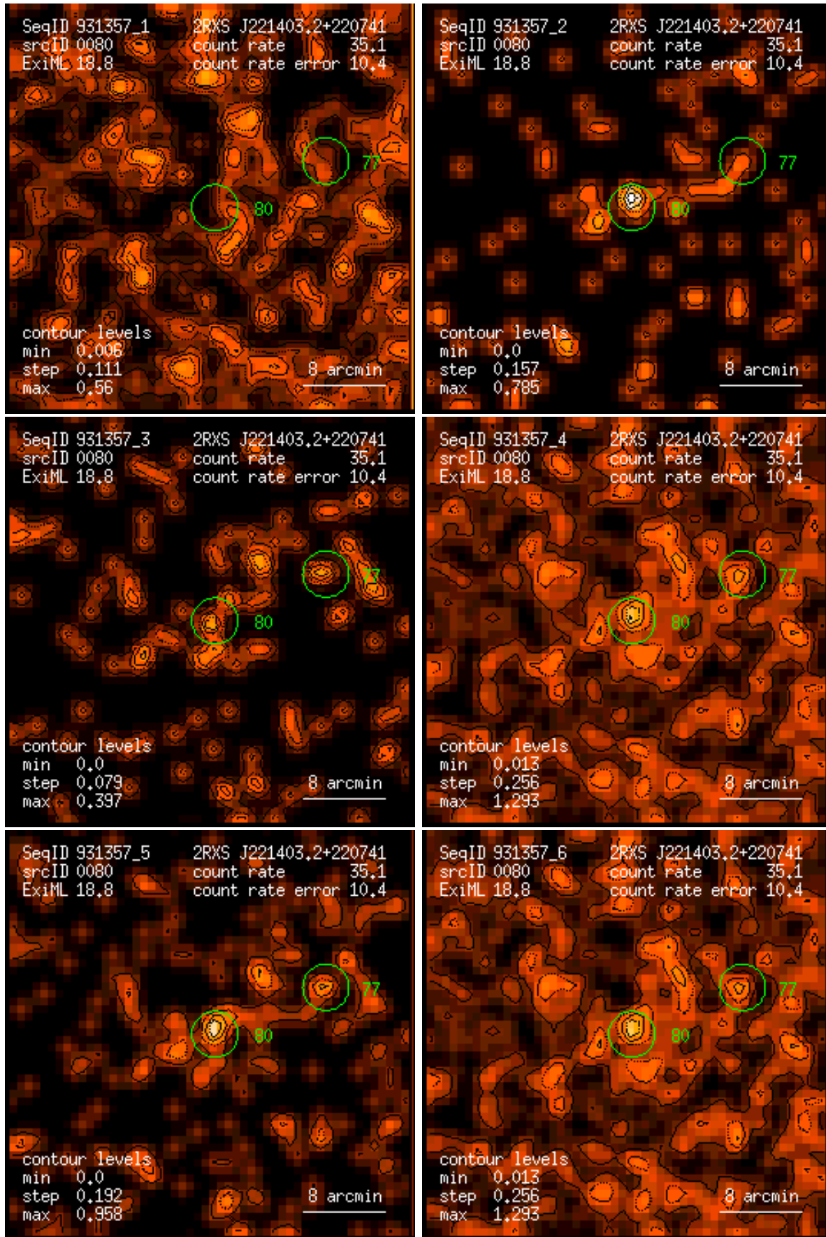
Figure 80: RASS 931357: detection 0080: band rate images, Gaussian filter: (1) PSPC channels 11 – 41, (2) 52 – 90, (3) 91 – 201, (4) 11 – 235, (5) 52 – 201, (6) 11 – 201. Broad band rates in counts/ks. Band rate contour levels in counts/ks/arcmin 2 .
