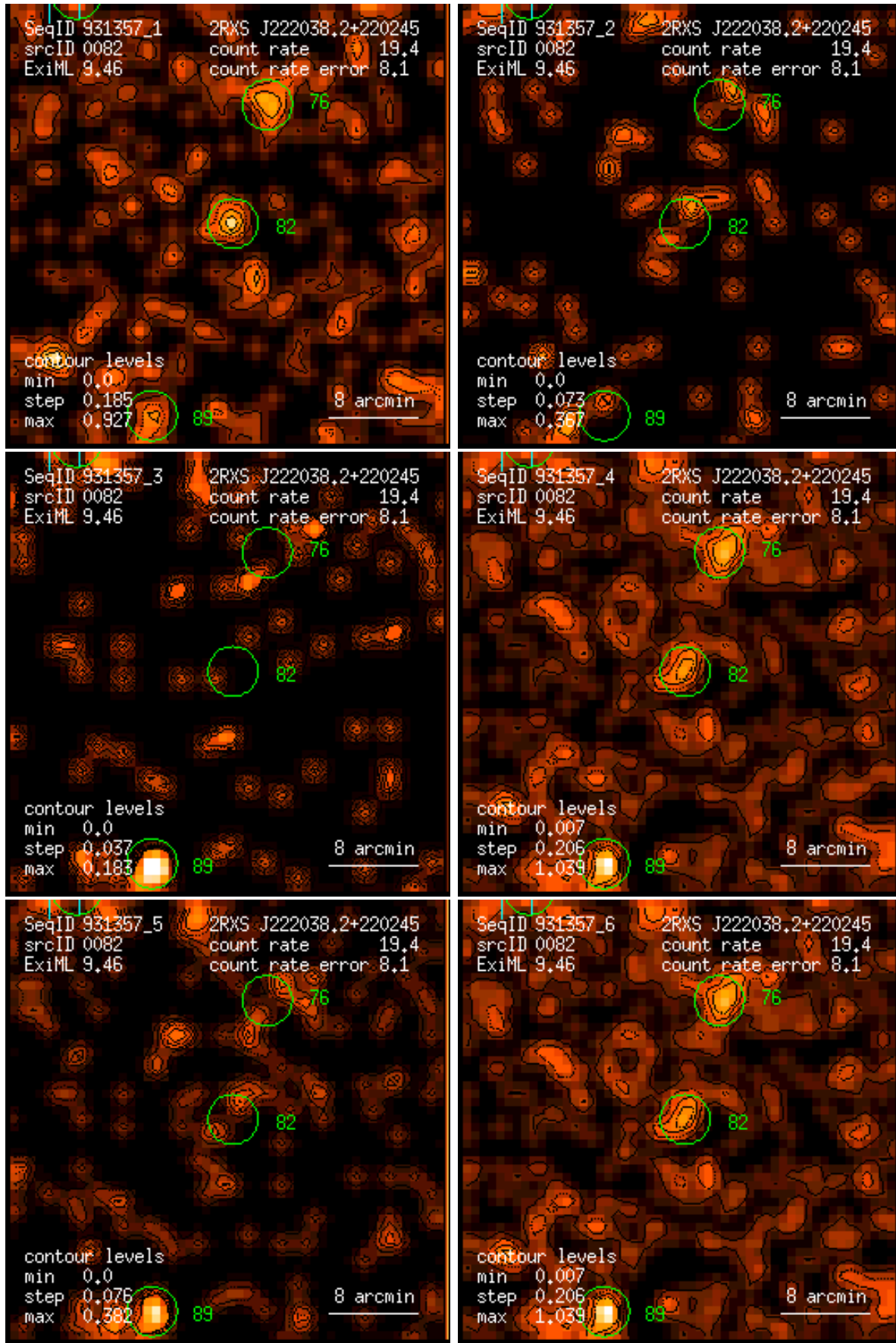
Figure 82: RASS 931357: detection 0082: band rate images, Gaussian filter: (1) PSPC channels 11 – 41, (2) 52 – 90, (3) 91 – 201, (4) 11 – 235, (5) 52 – 201, (6) 11 – 201. Broad band rates in counts/ks. Band rate contour levels in counts/ks/arcmin 2 .
