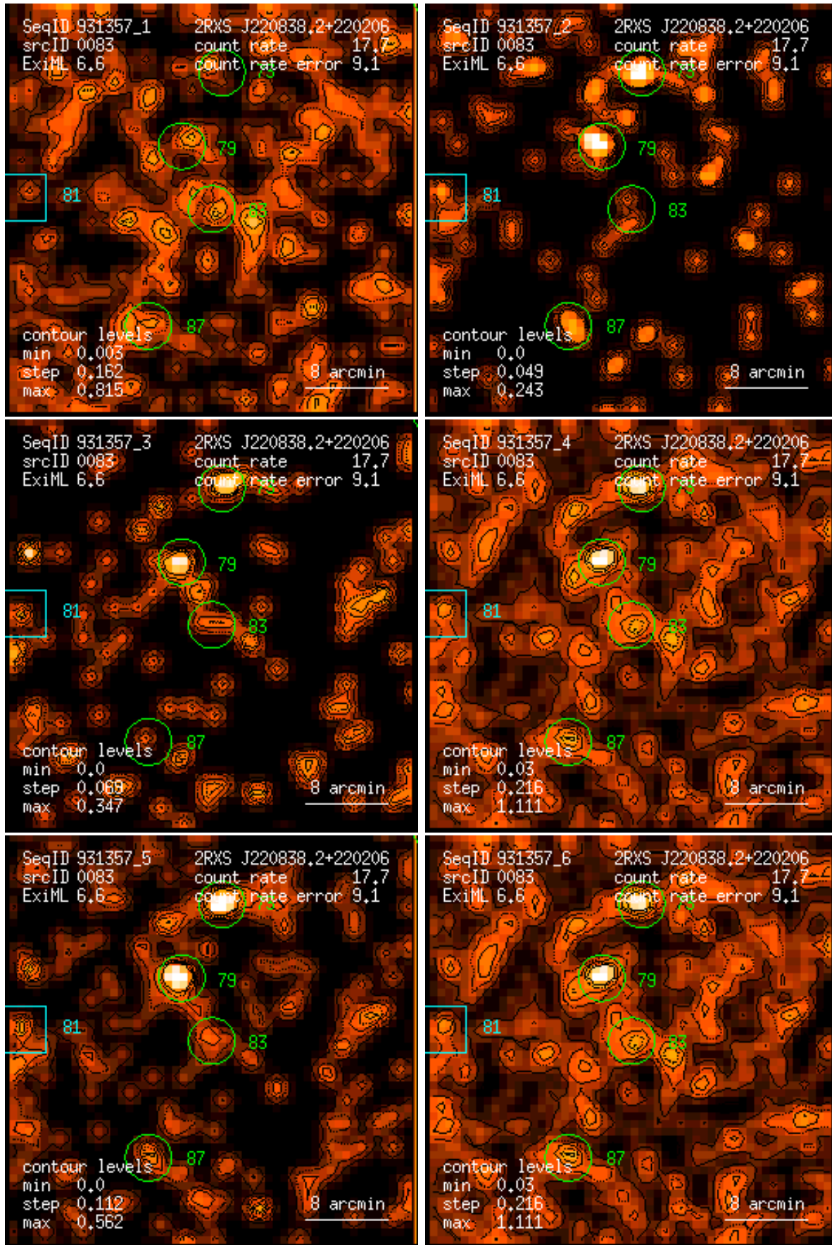
Figure 83: RASS 931357: detection 0083: band rate images, Gaussian filter: (1) PSPC channels 11 – 41, (2) 52 – 90, (3) 91 – 201, (4) 11 – 235, (5) 52 – 201, (6) 11 – 201. Broad band rates in counts/ks. Band rate contour levels in counts/ks/arcmin 2 .
