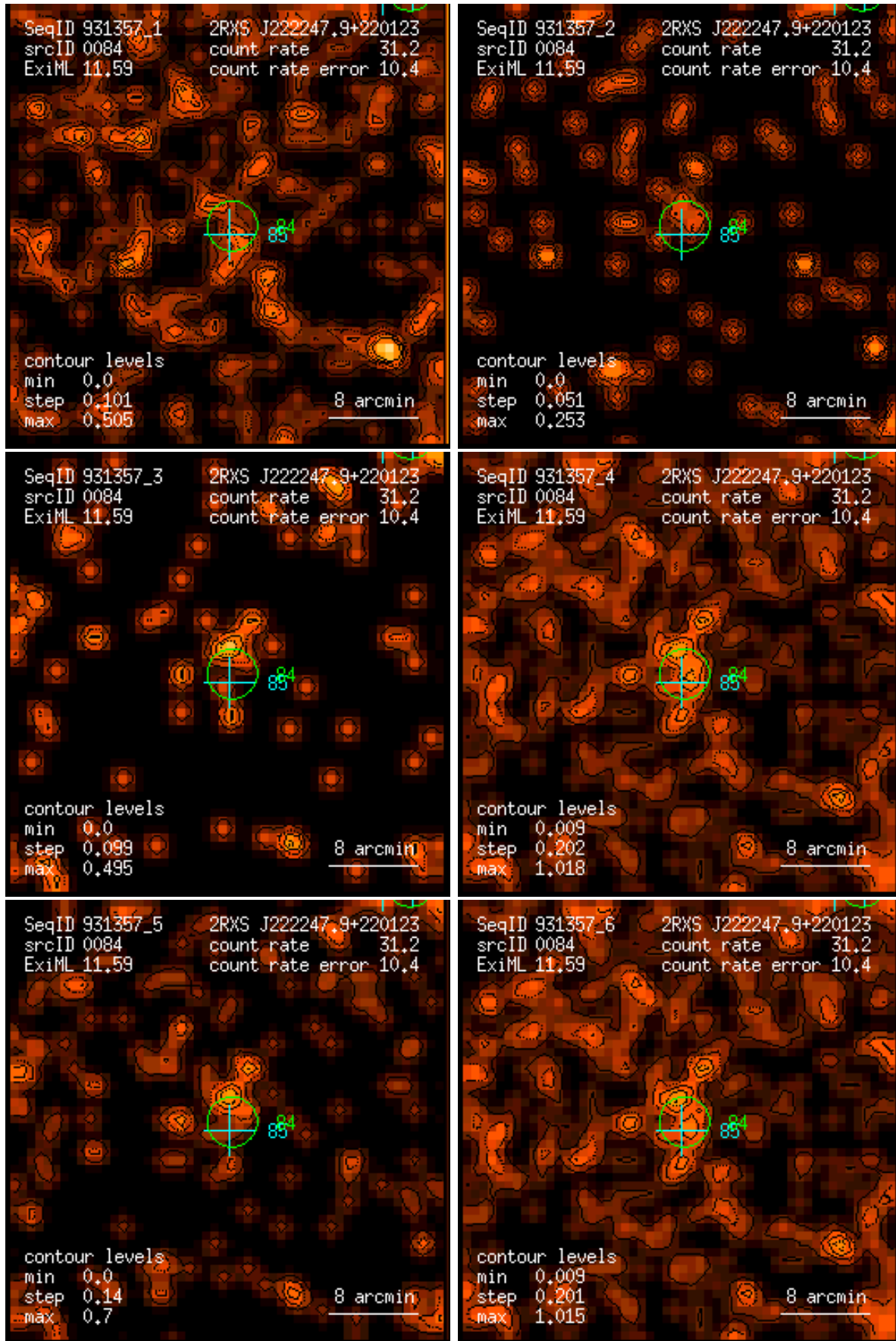
Figure 84: RASS 931357: detection 0084: band rate images, Gaussian filter: (1) PSPC channels 11 – 41, (2) 52 – 90, (3) 91 – 201, (4) 11 – 235, (5) 52 – 201, (6) 11 – 201. Broad band rates in counts/ks. Band rate contour levels in counts/ks/arcmin 2 .
