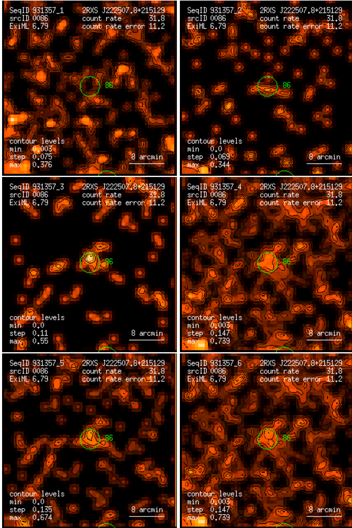
Figure 86: RASS 931357: detection 0086: band rate images, Gaussian filter: (1) PSPC channels 11 – 41, (2) 52 – 90, (3) 91 – 201, (4) 11 – 235, (5) 52 – 201, (6) 11 – 201. Broad band rates in counts/ks. Band rate contour levels in counts/ks/arcmin 2 .
